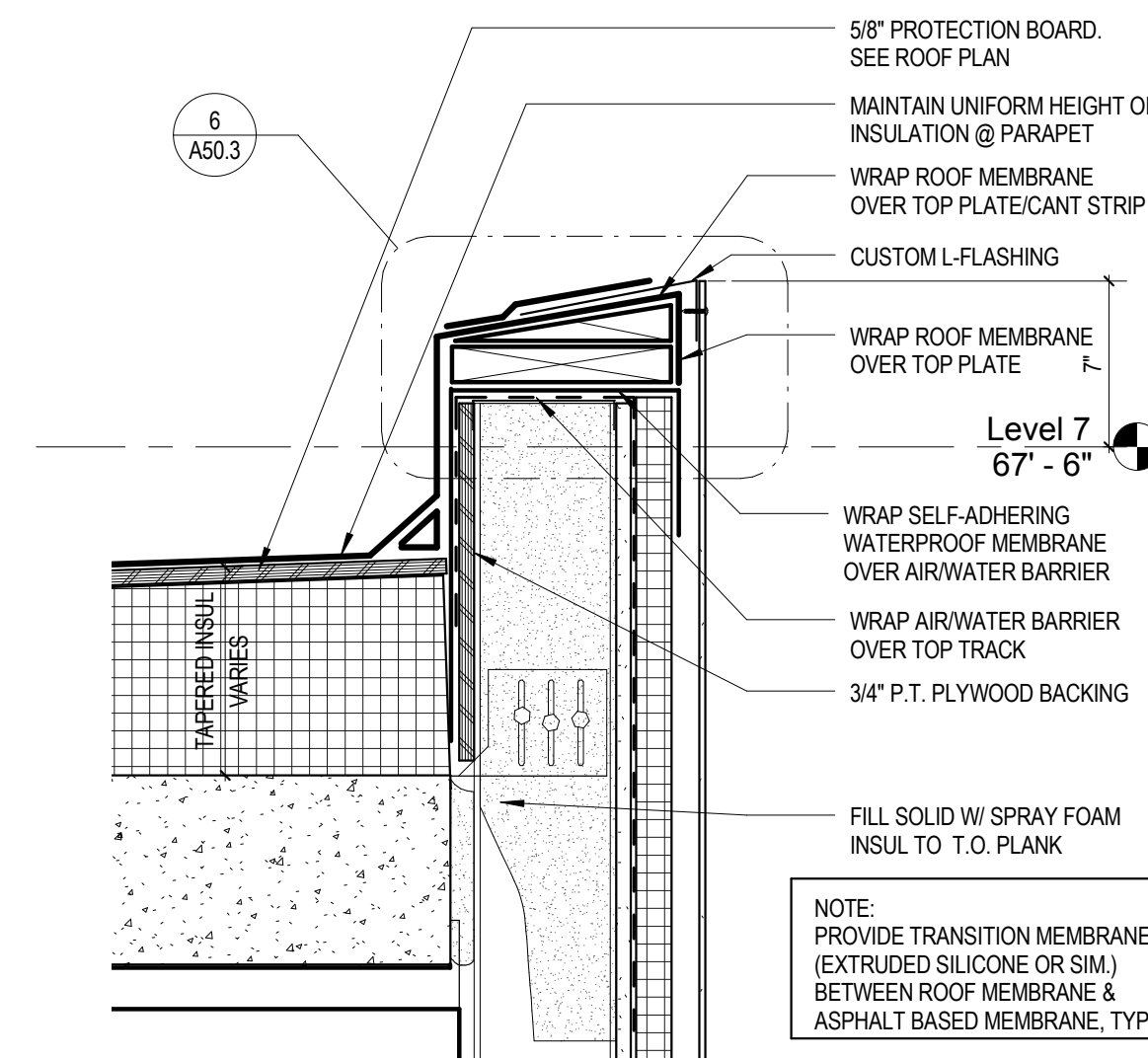
6 DETAIL LEVEL 7 PARAPET 1 1/2" = 1'-0"
