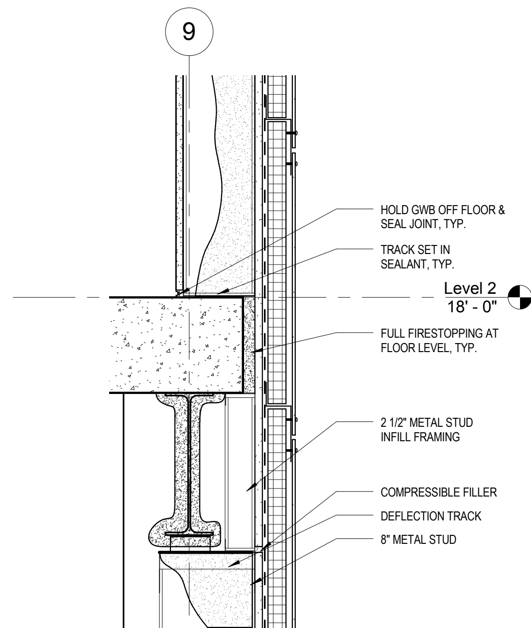
8 DETAIL EAST WALL LEVEL 2 1 1/2" = 1'-0"
