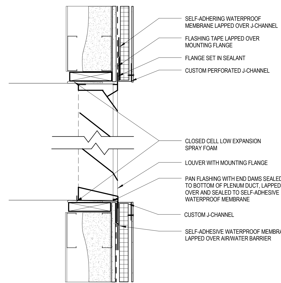
5 DETAIL WALL SECTION LOUVER, TYP. 1 1/2" = 1'-0"
