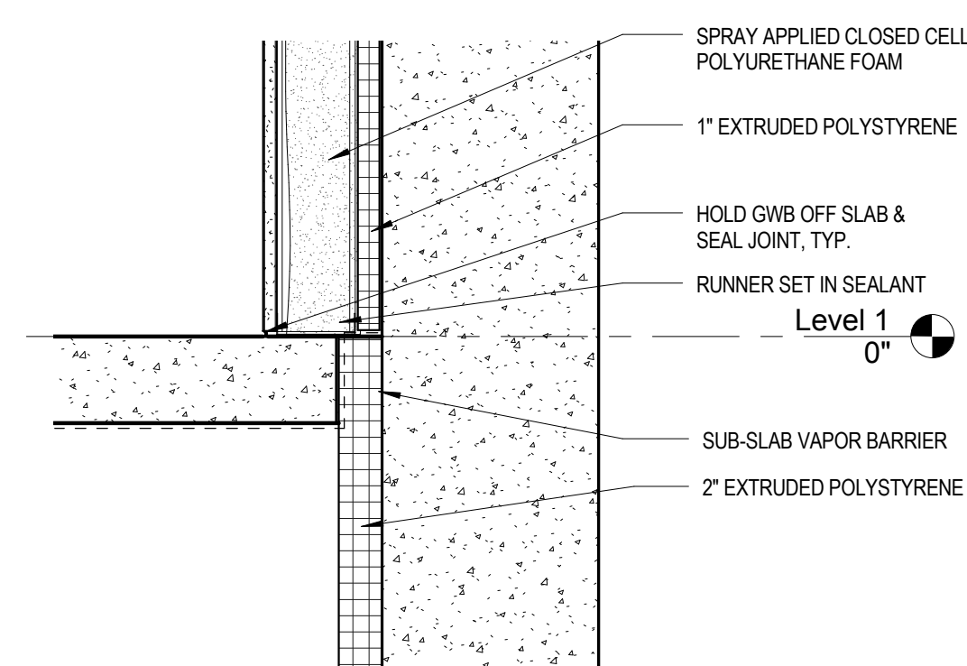
7 DETAIL FOUNDATION w/ INTERIOR PARTITION 1 1/2" = 1'-0"
