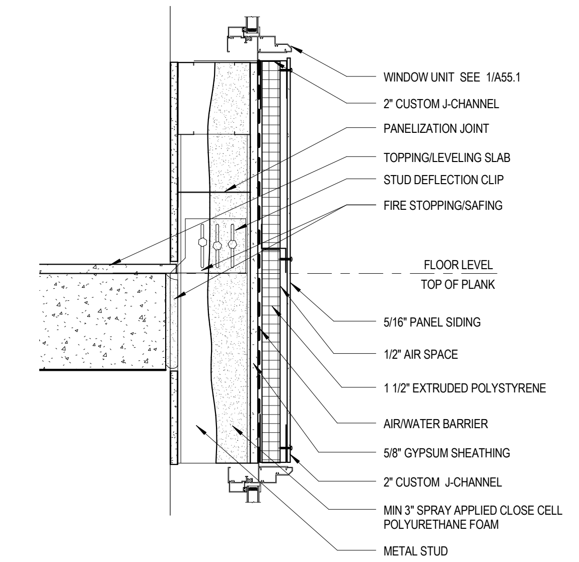
2 DETAIL PANEL SIDING WINDOW TYP 1 1/2" = 1'-0"
