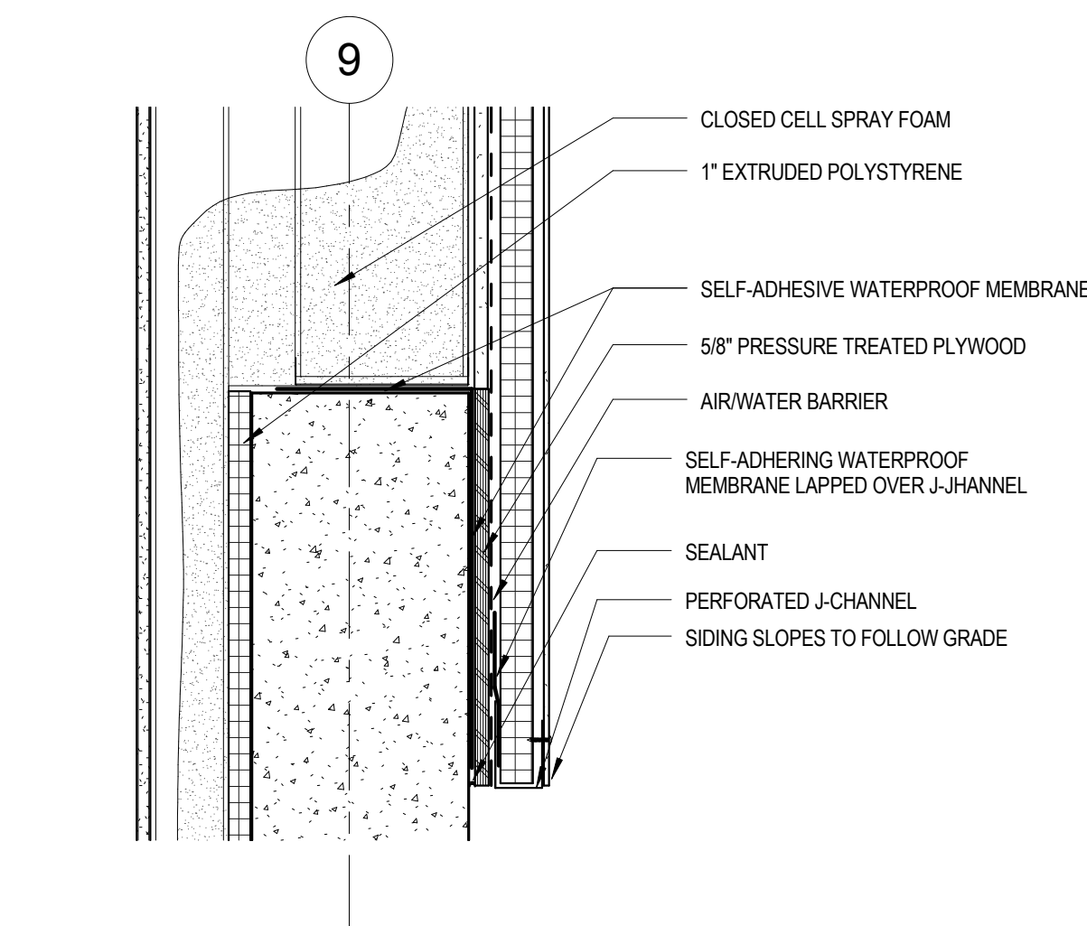
10 DETAIL BASE OF EAST WALL 1 1/2" = 1'-0"
