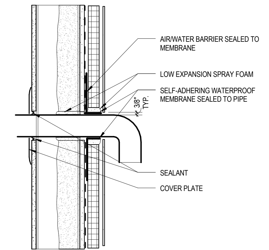
3 DETAIL PANEL SIDING PENETRATION, TYP. 1 1/2" = 1'-0"
