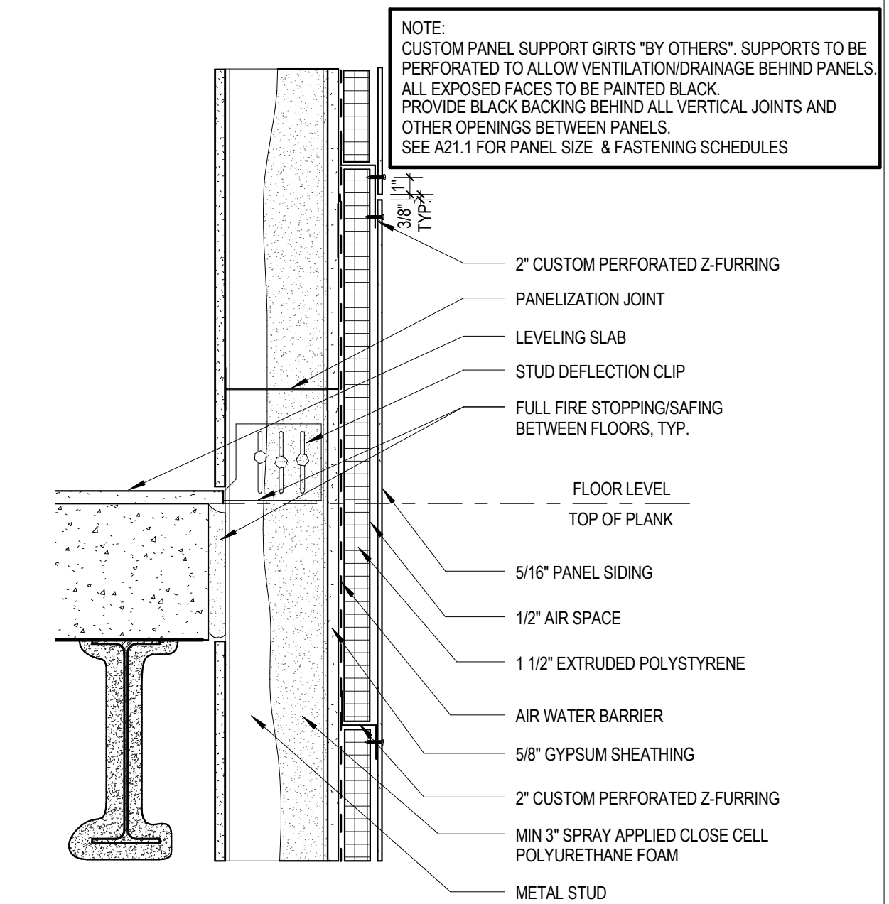
1 DETAIL PANEL SIDING WALL SECTION TYP 1 1/2" = 1'-0"
