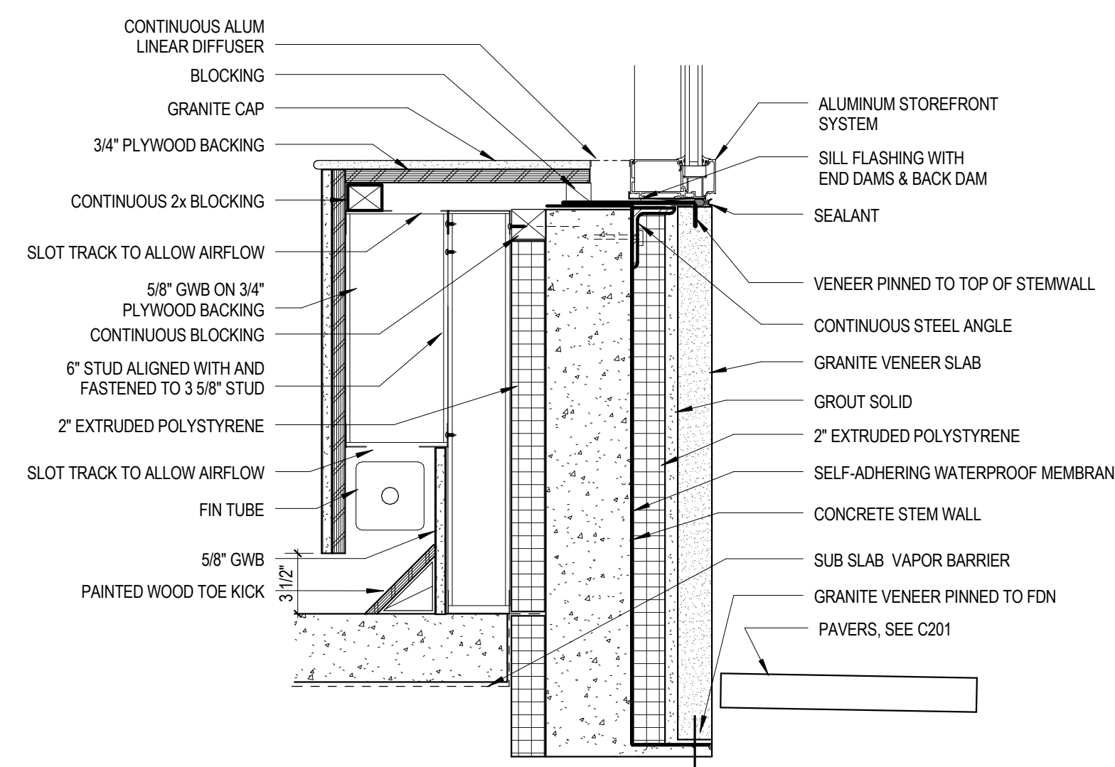
4 DETAIL BASE OF WALL STOREFRONT 1 1/2" = 1'-0"
