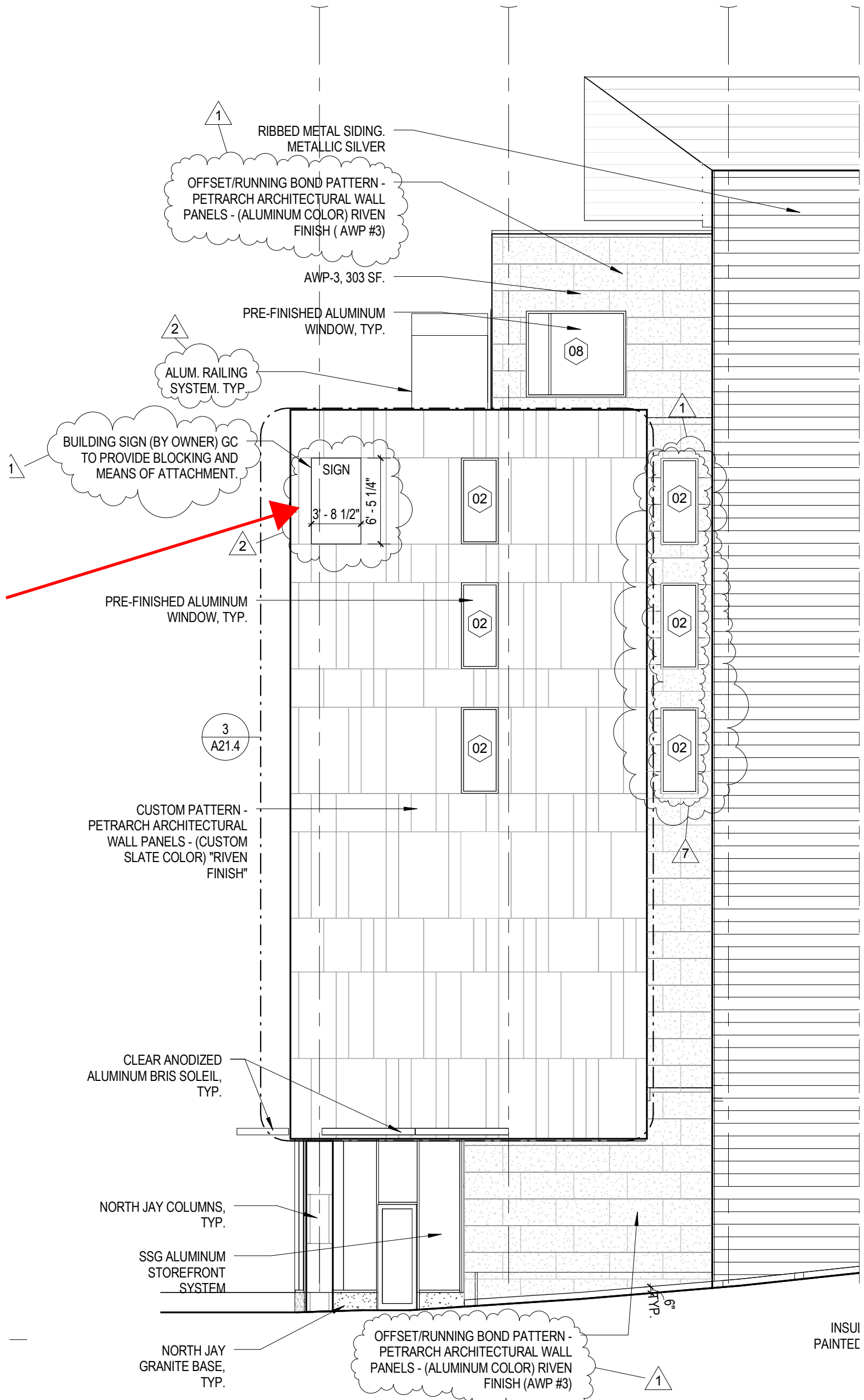
1 EAST ELEVATION 1/8" = 1'-0"
