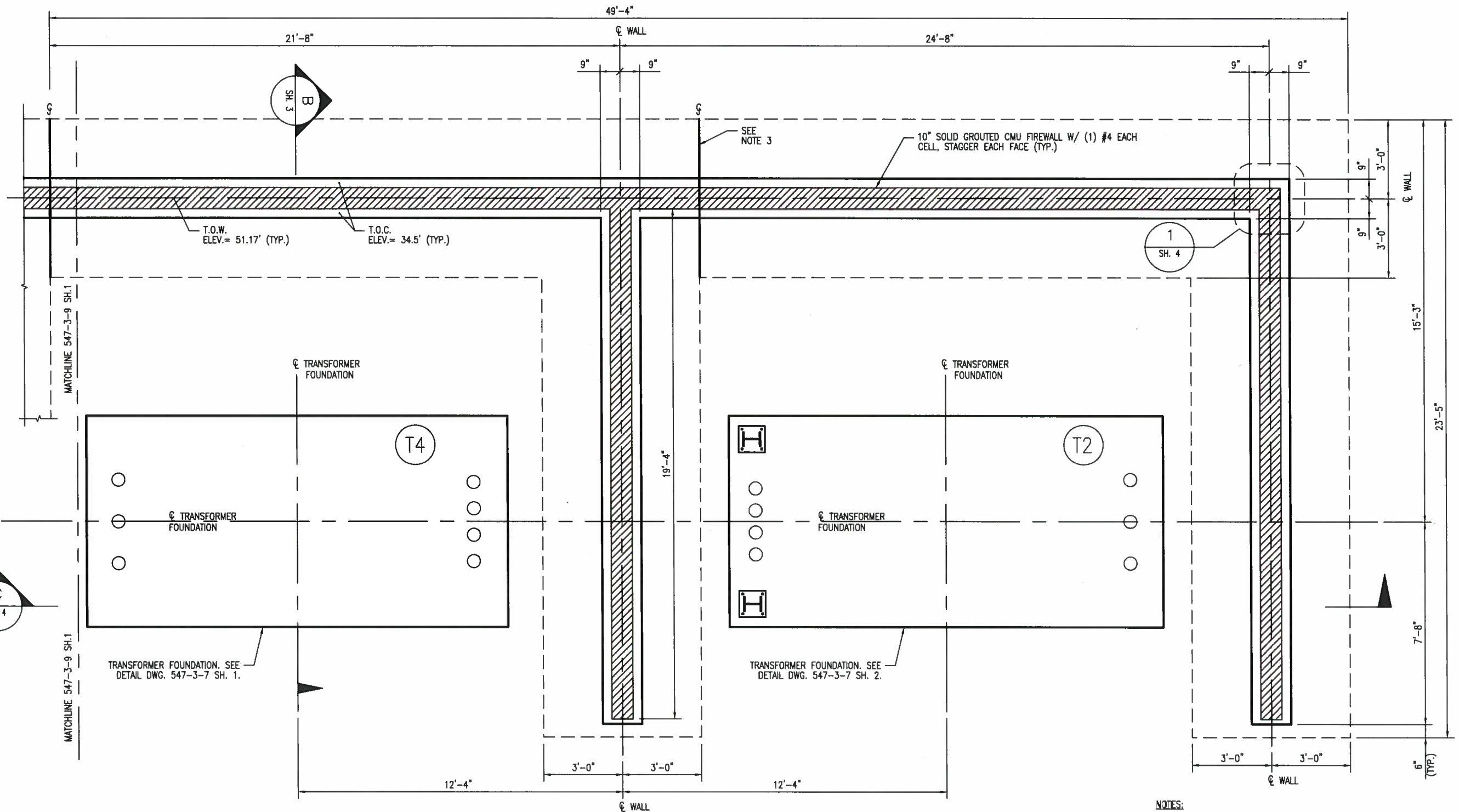
FIREWALL FOUNDATION PLAN SCALE: 1/4" = 1'-0"
