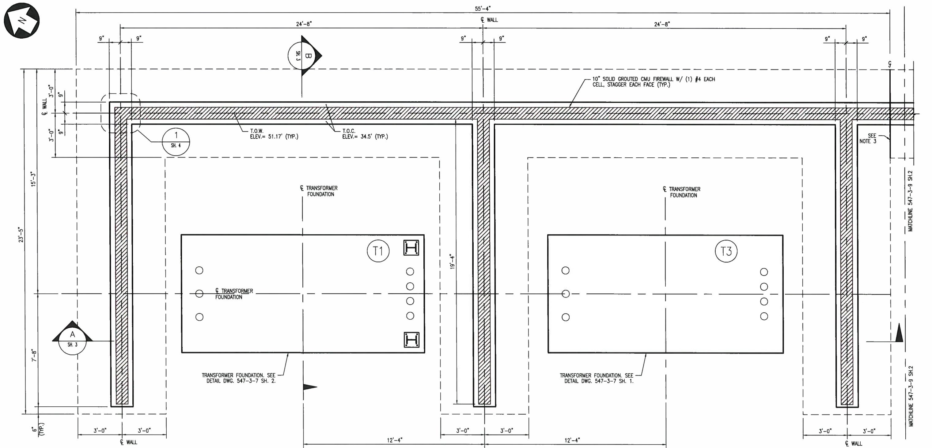
FIREWALL FOUNDATION PLAN SCALE: 1/4" = 1'-0"
