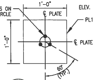
1 DETAIL 1 547-3-8 SH.1 SCALE: 3/4"=1'-0"
