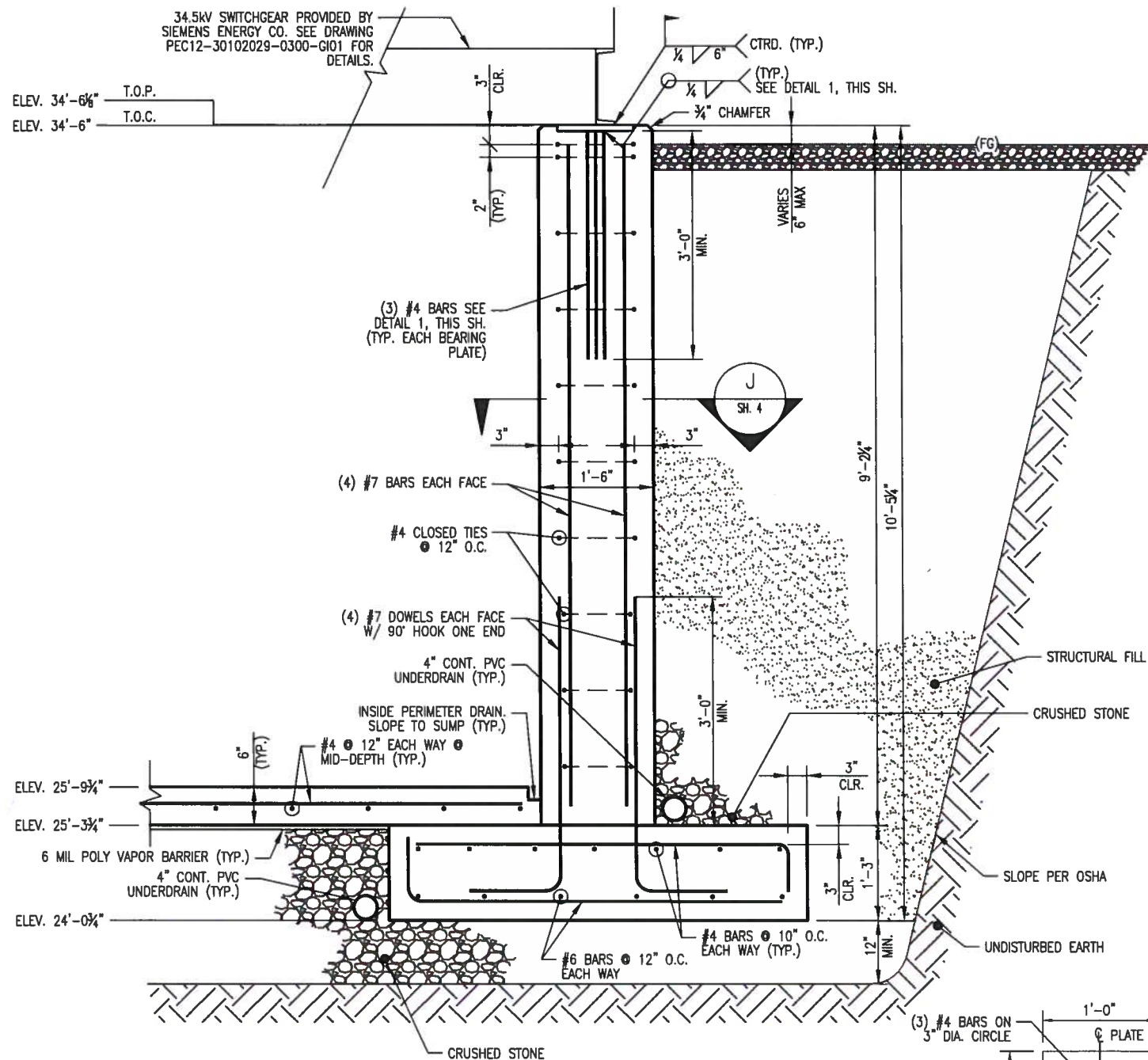
B SECTION B 547-3-8 SH.1 SCALE: 1/2"=1'-0"
