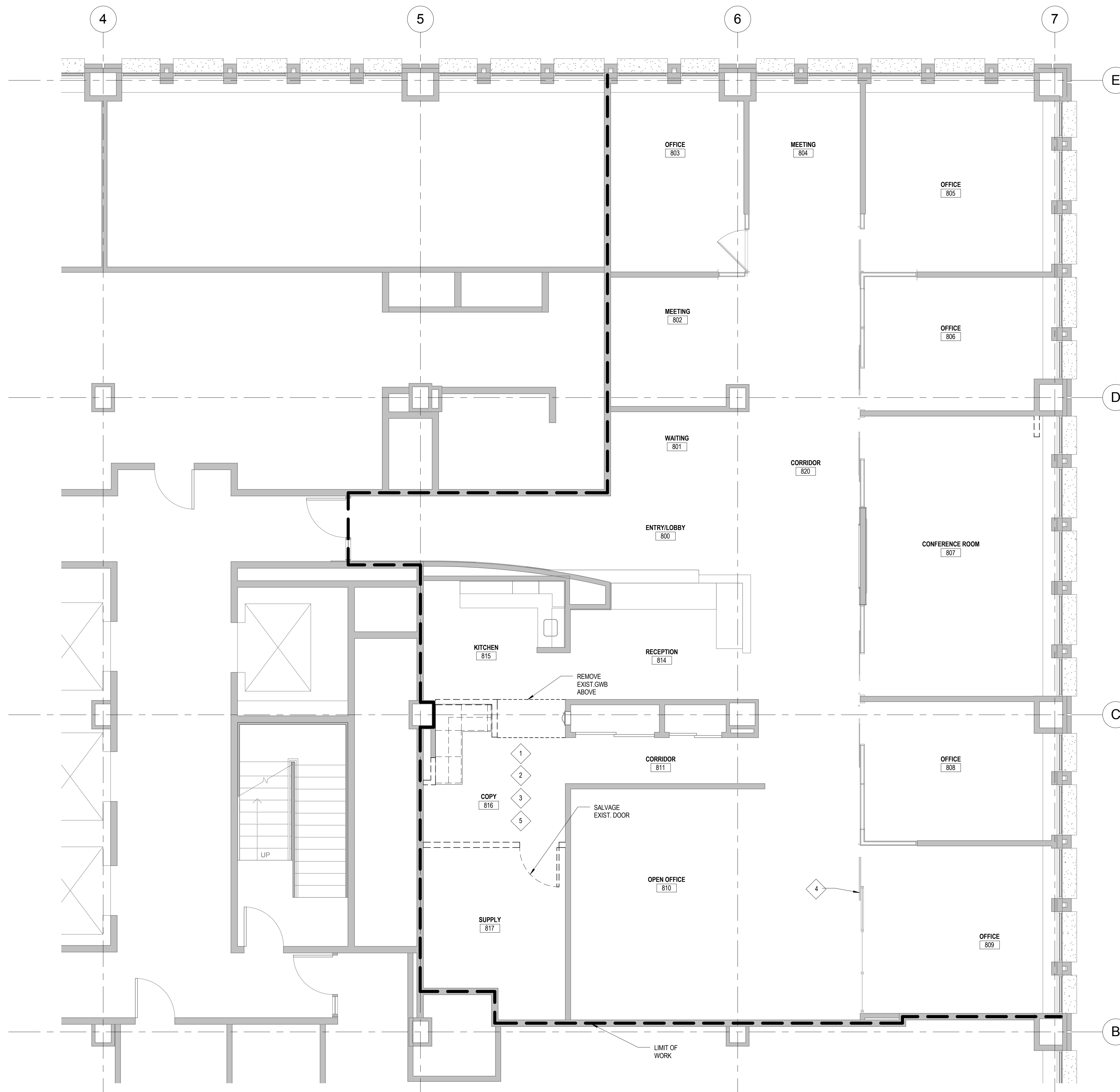
1 DEMOLITION PLAN 1/4" = 1'-0"
