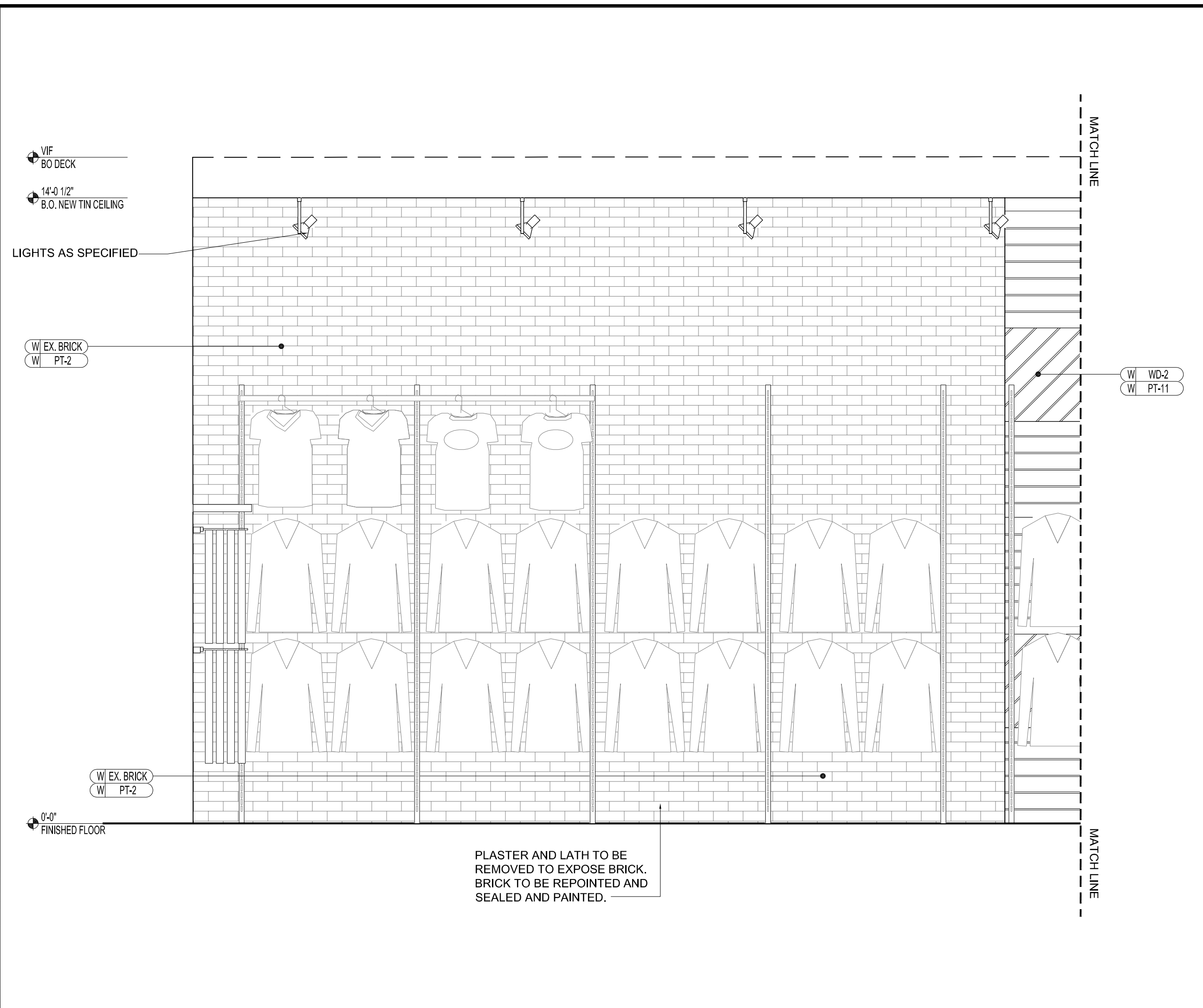
2 INTERIOR ELEVATION SCALE: 1/2" = 1'-0"
