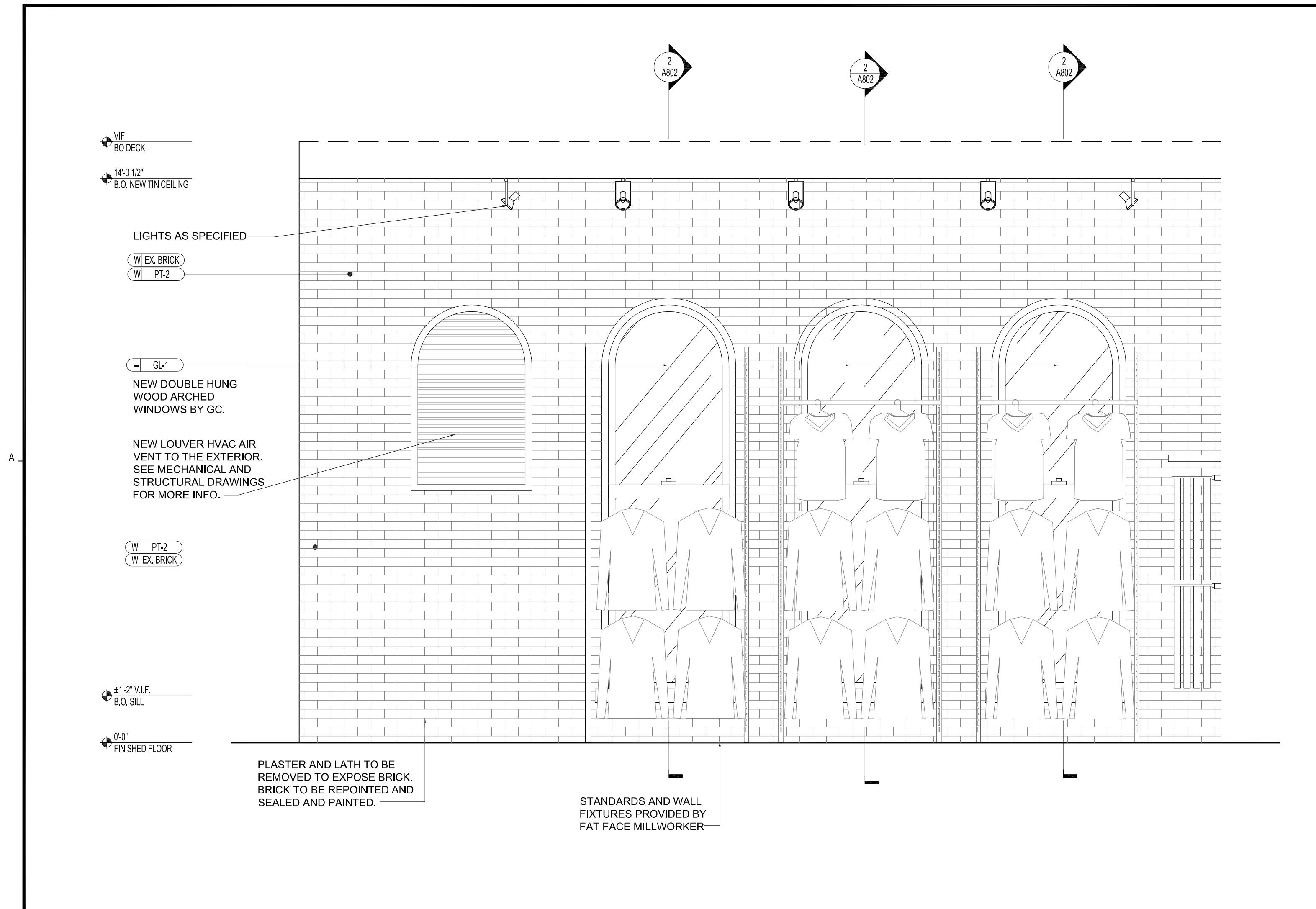
1 INTERIOR ELEVATION SCALE: 1/2" = 1'-0"
