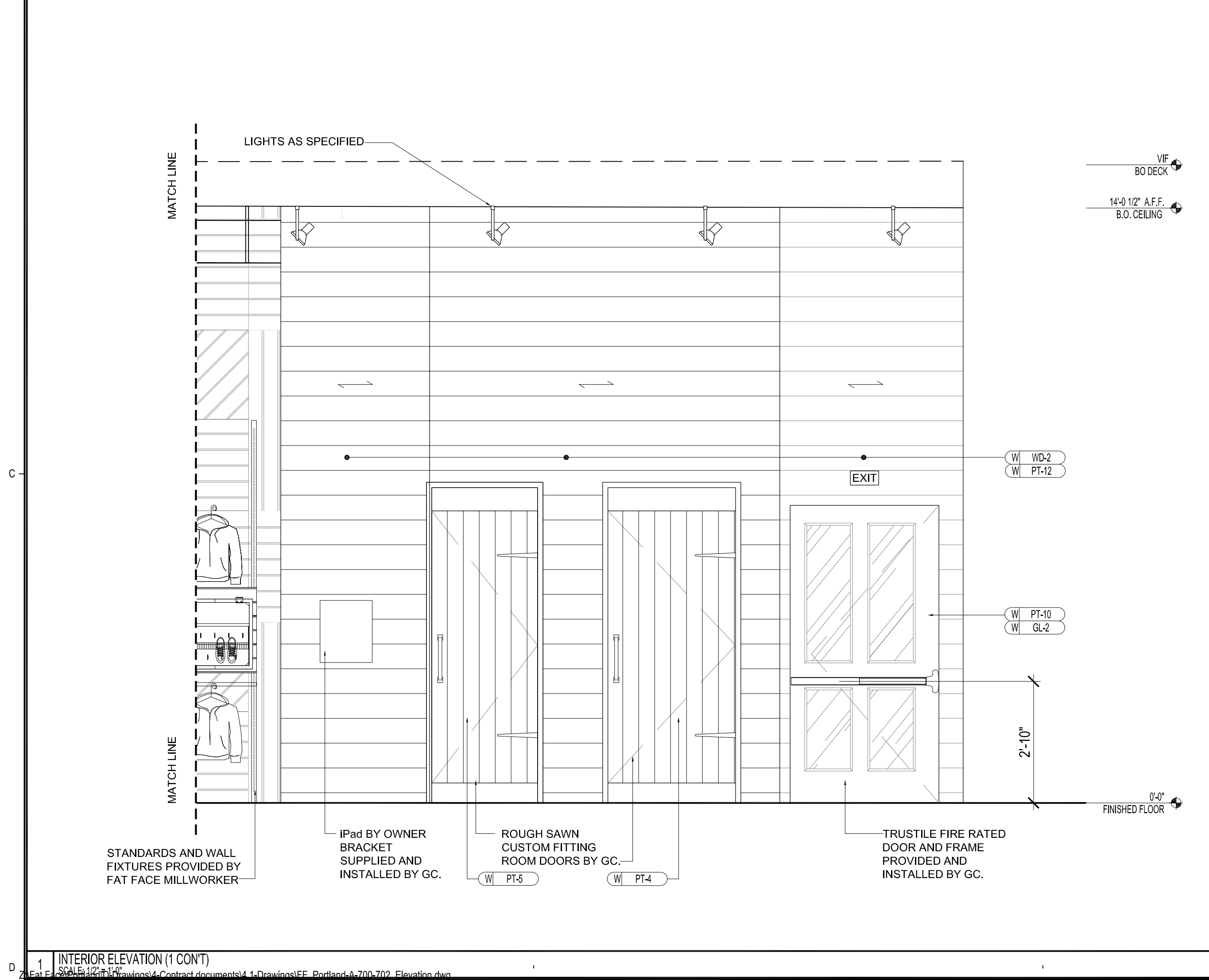
1 INTERIOR ELEVATION (1 CONT) SCALE: 1/2" = 1'-0"
