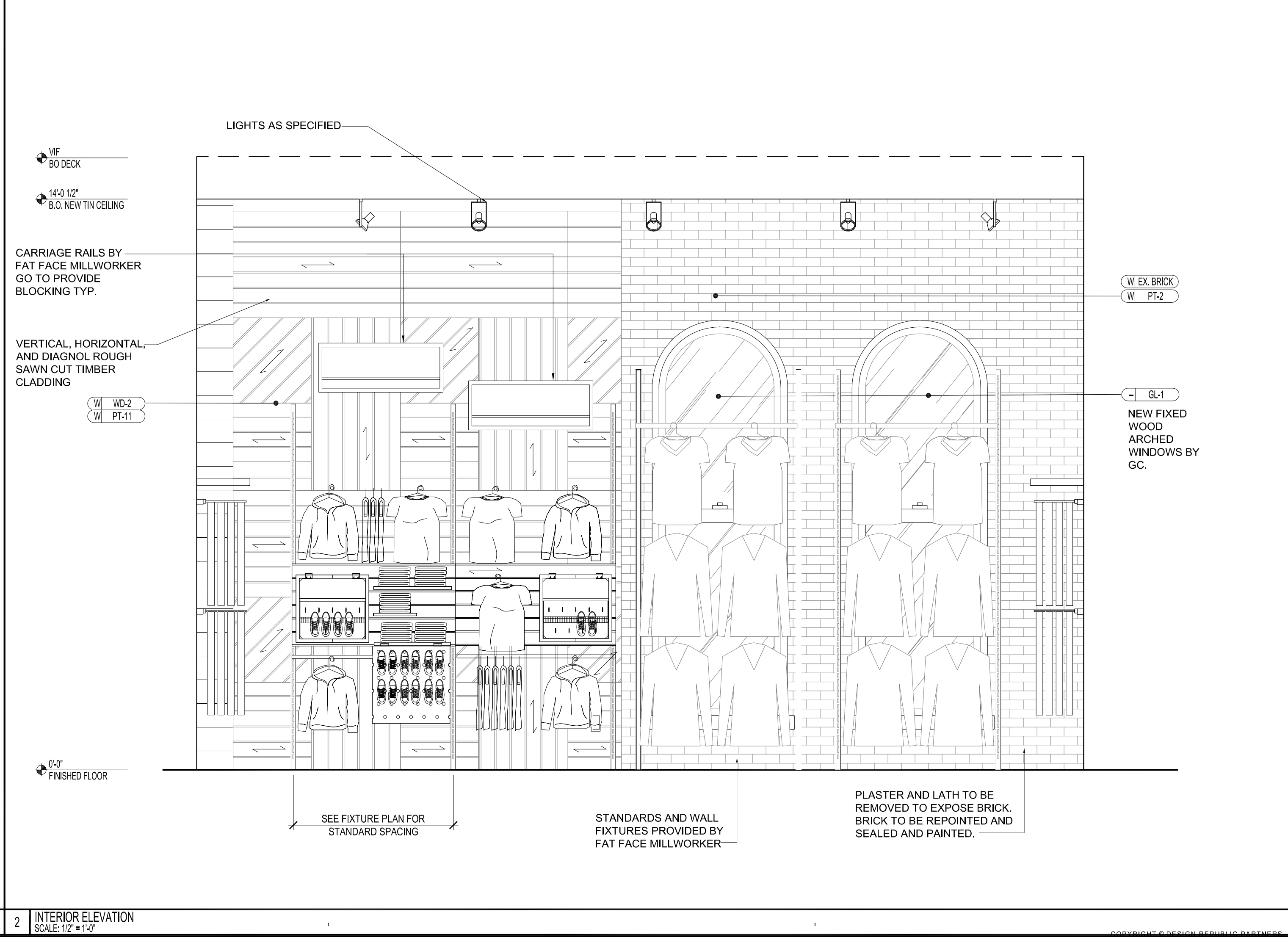
2 INTERIOR ELEVATION SCALE: 1/2" = 1'-0"
