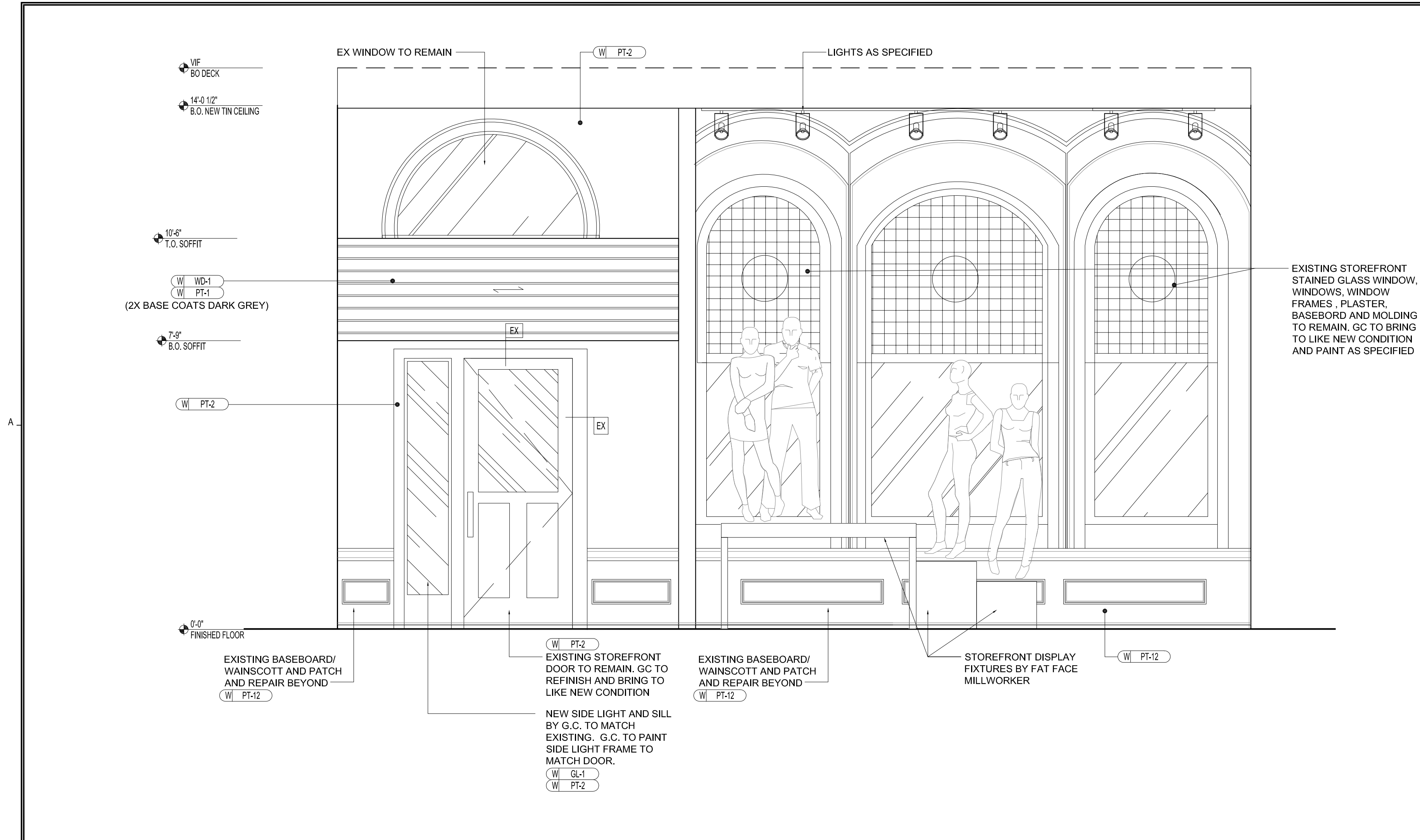
1 INTERIOR ELEVATION SCALE: 1/2" = 1'-0"
