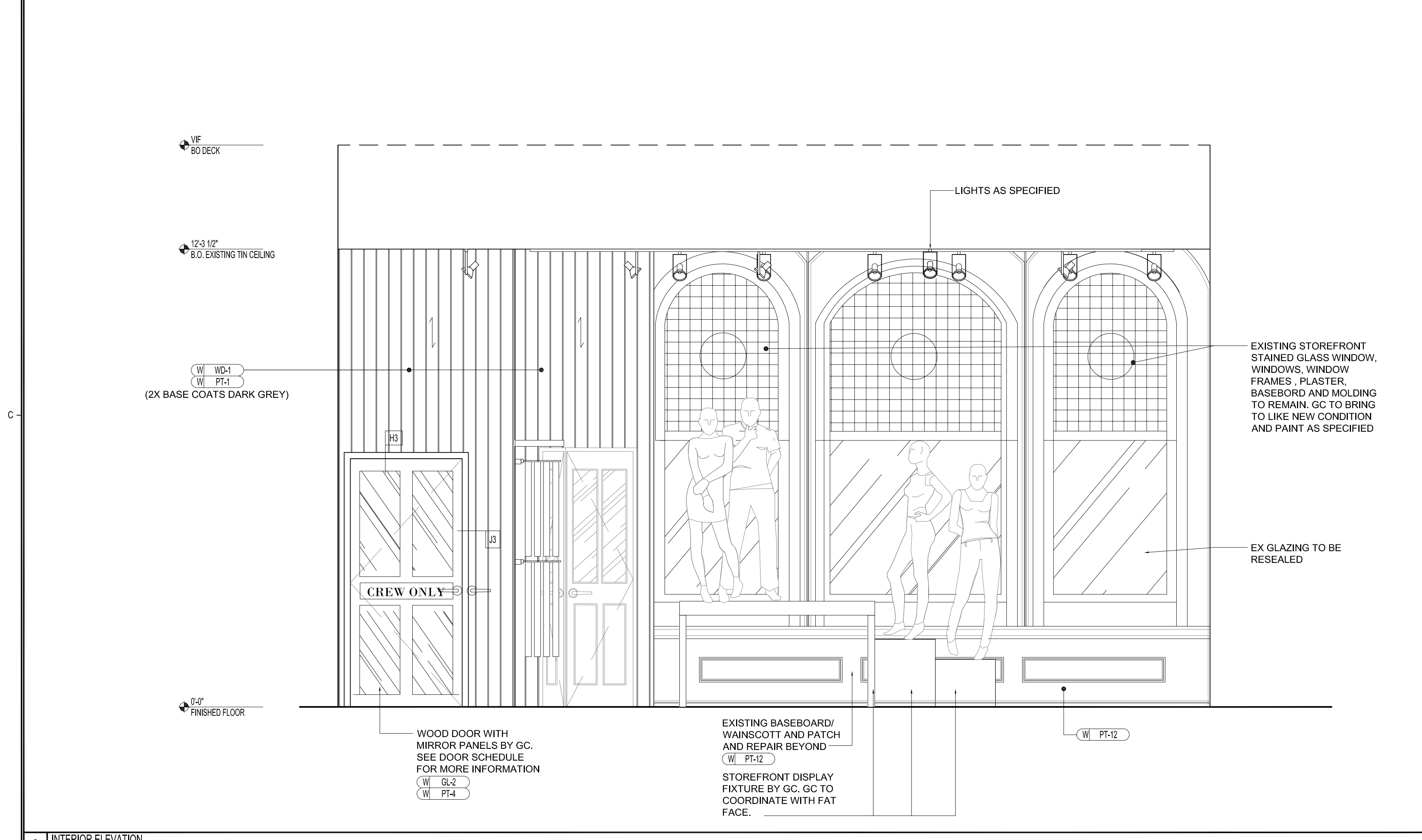
2 INTERIOR ELEVATION SCALE: 1/2" = 1'-0"
