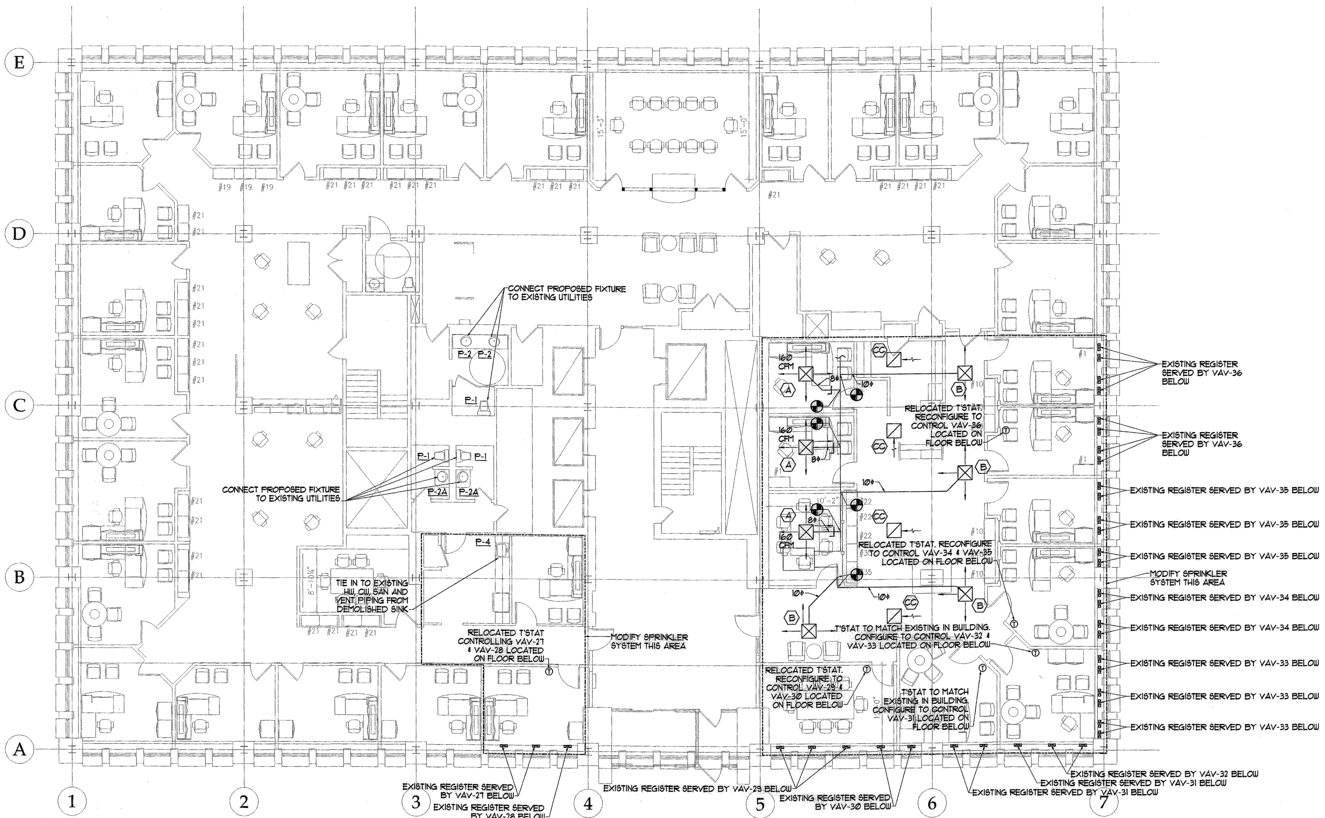
SECOND FLOOR MECHANICAL PLAN SCALE - 1/8" = 1' - 0"
