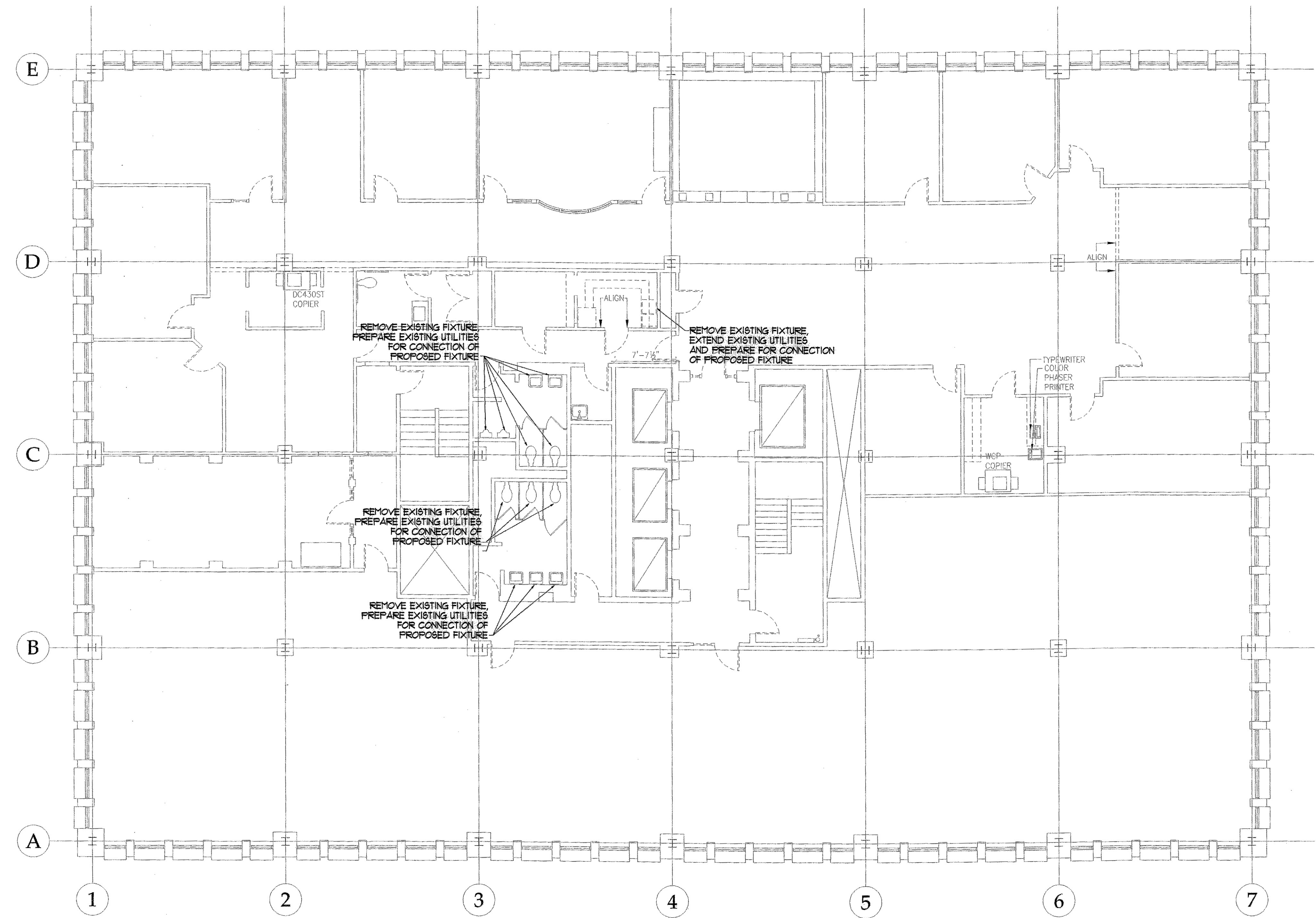
SEVENTH FLOOR MECHANICAL DEMOLITION PLAN SCALE - 1/8" = 1' - 0"
