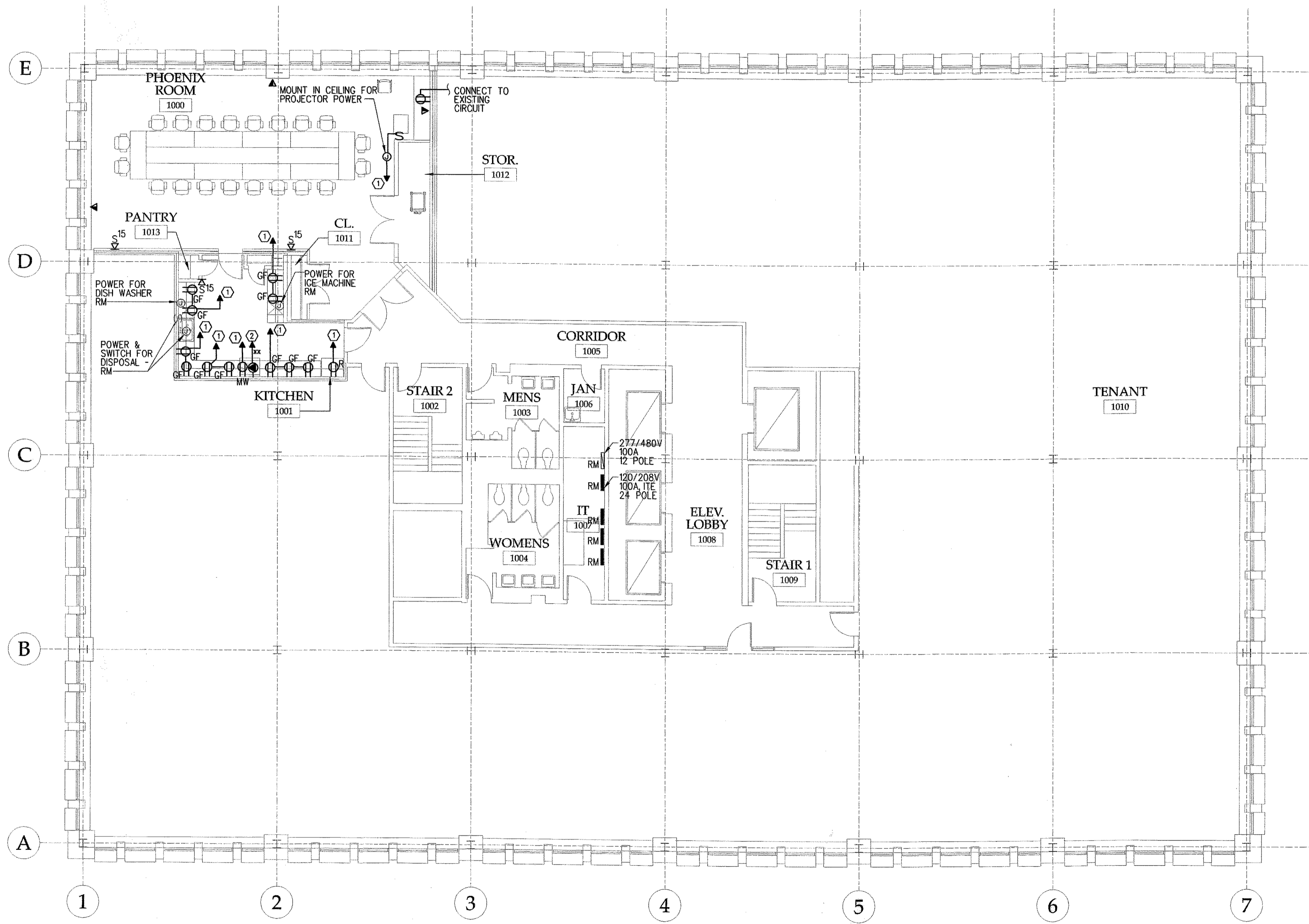
TENTH FLOOR POWER PLAN SCALE - 1/8" = 1' - 0"
