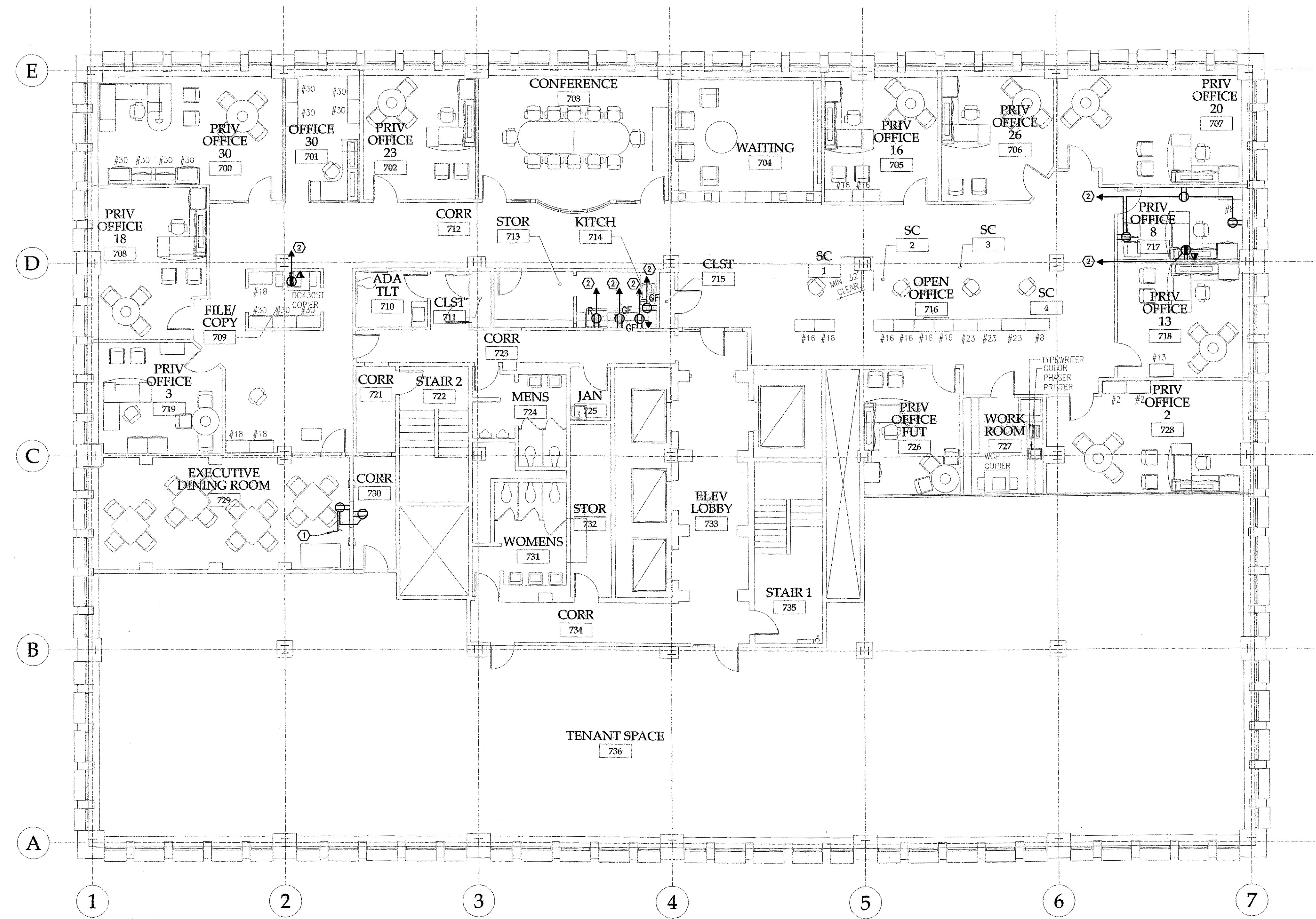
SEVENTH FLOOR POWER PLAN SCALE - 1/8" = 1' - 0"
