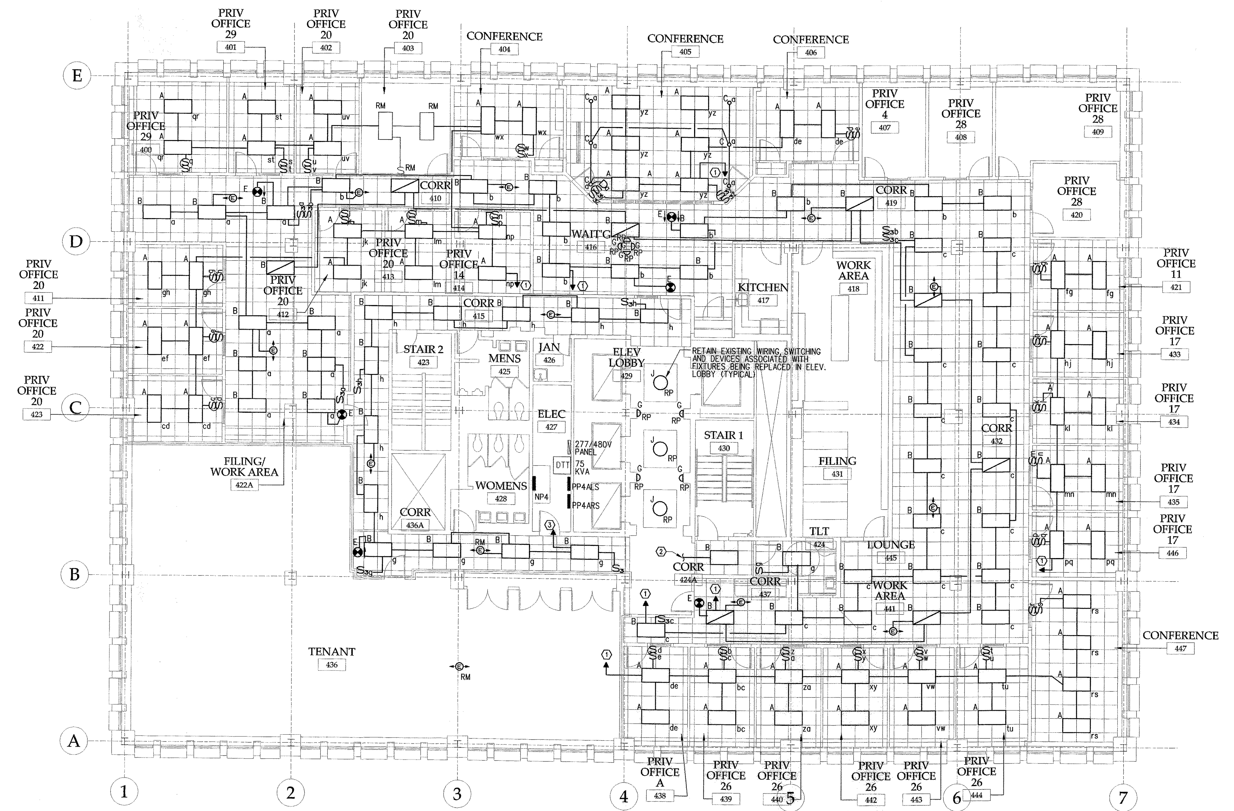
FOURTH FLOOR LIGHTING PLAN SCALE - 1/8" = 1' - 0"
