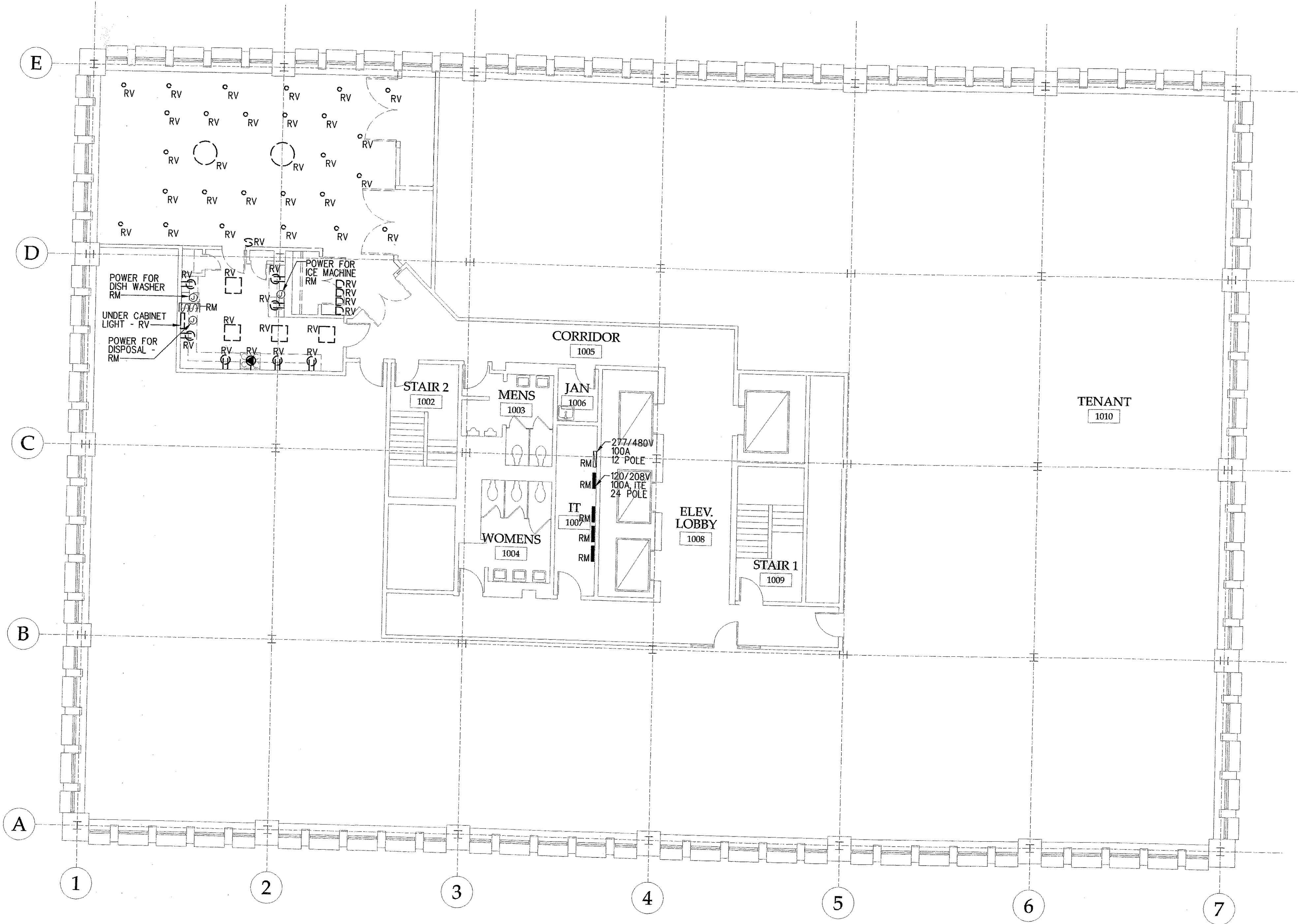
TENTH FLOOR ELECTRICAL DEMOLITION PLAN SCALE - 1/8" = 1' - 0"
