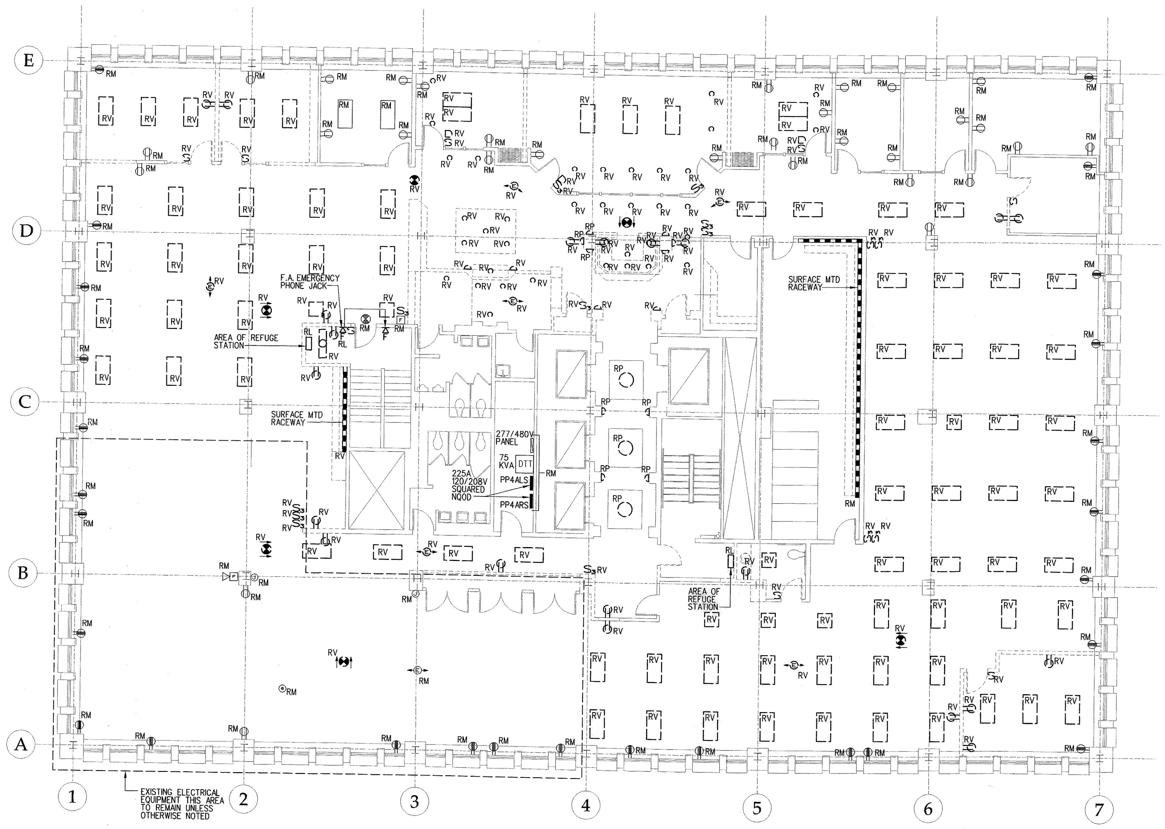
FOURTH FLOOR ELECTRICAL DEMOLITION PLAN SCALE - 1/8" = 1' - 0"
