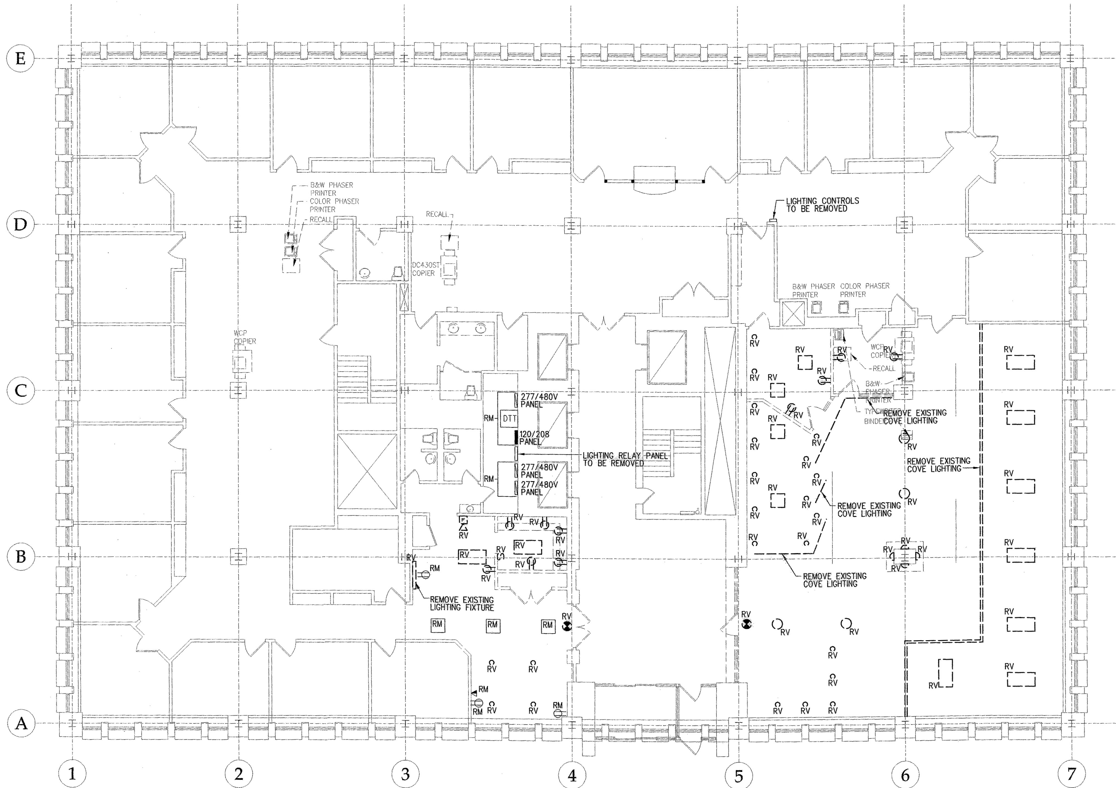
SECOND FLOOR ELECTRICAL DEMO PLAN SCALE - 1/8" = 1' - 0"
