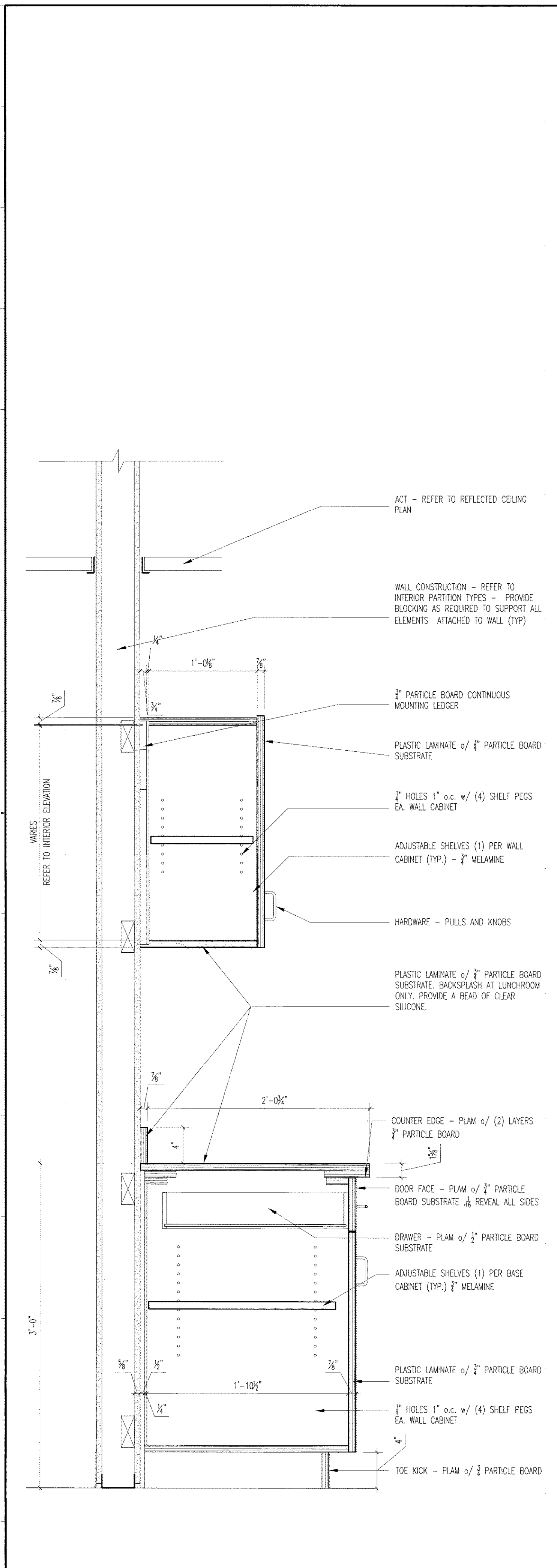
A1 HIGH PRESSURE LAMINATE CABINET DETAIL 1/2"=1'-0" CANAL PLAZA
