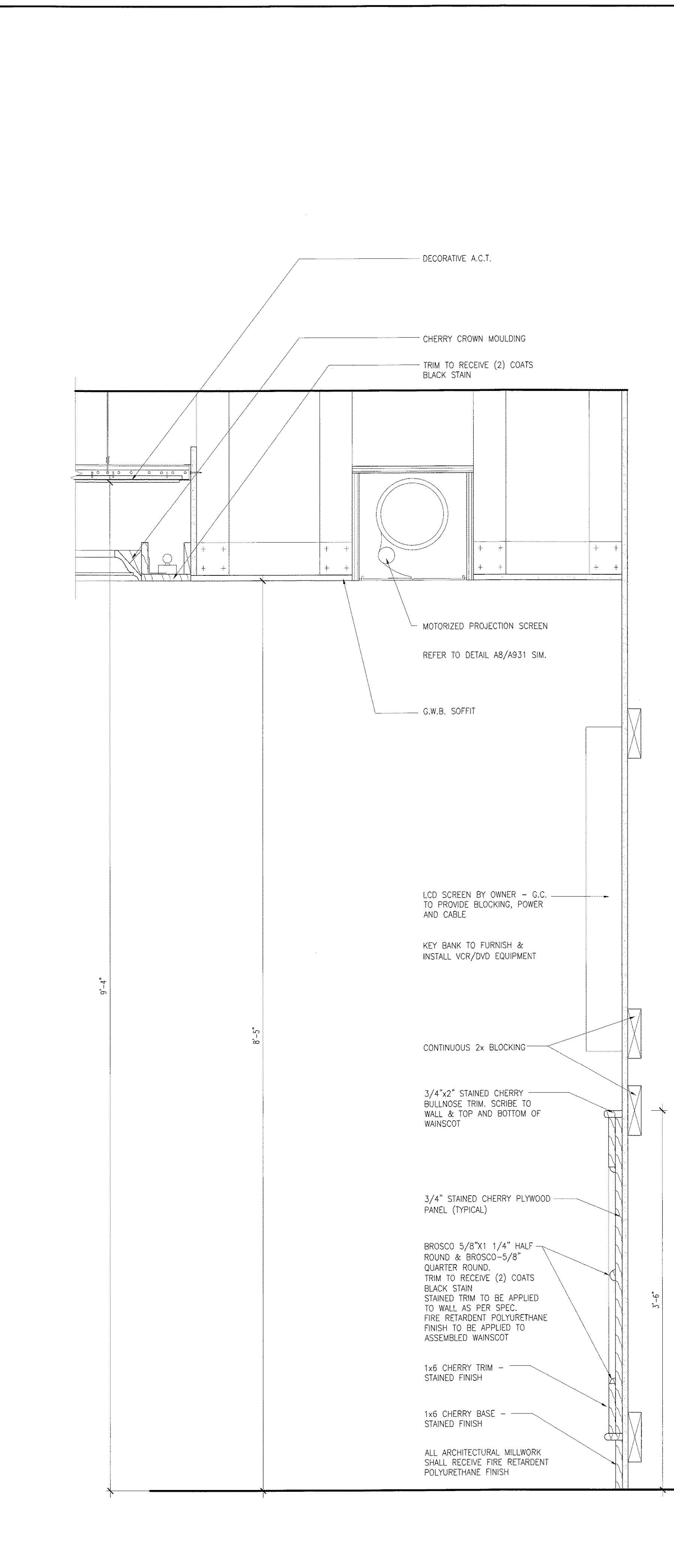
A11 WAINSCOT DETAIL @ PHOENIX ROOM 1/2"=1'-0" CANAL PLAZA, TENTH FLOOR
