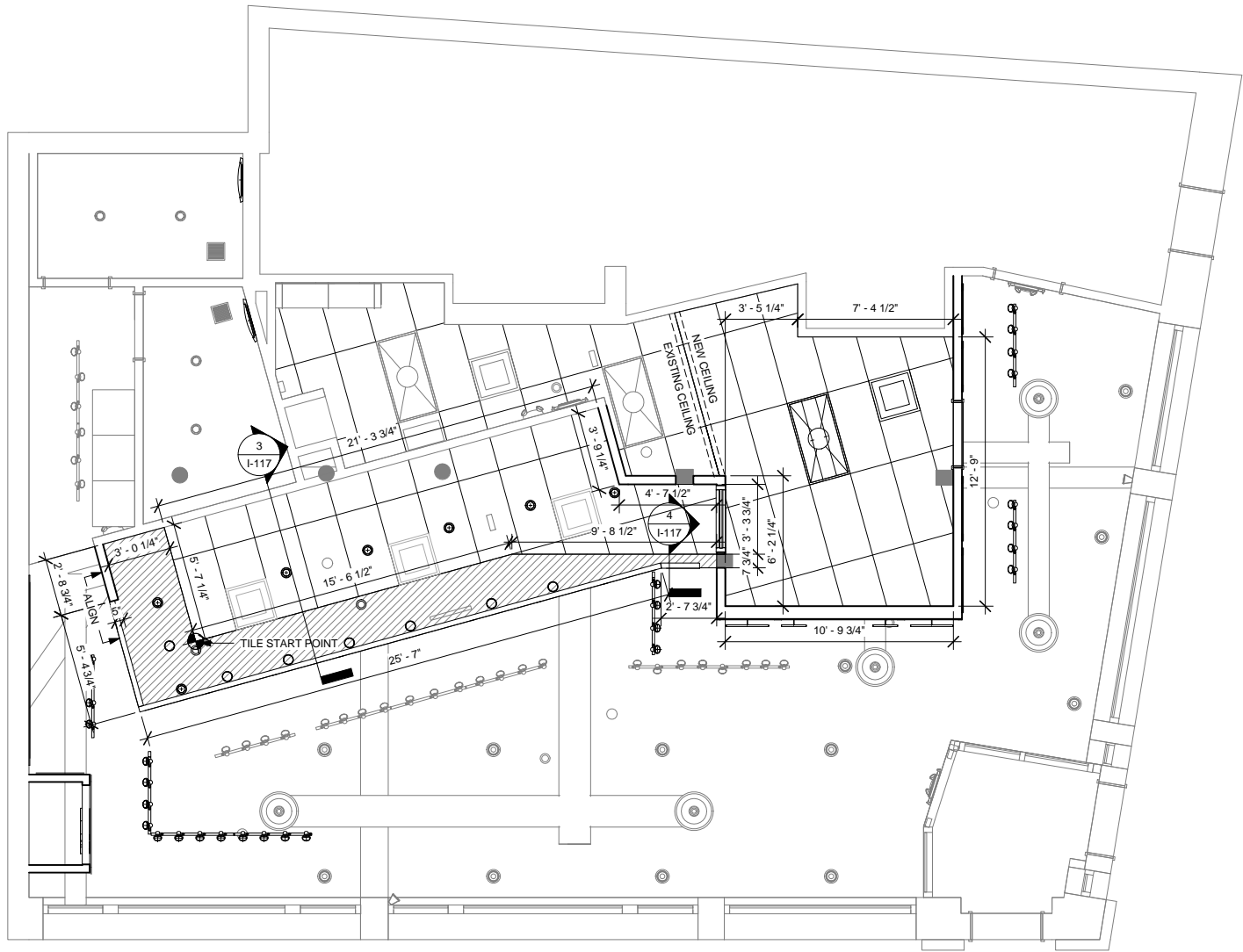
1 DIMENSIONED CEILING PLAN Scale: 1/4" = 1'-0"
