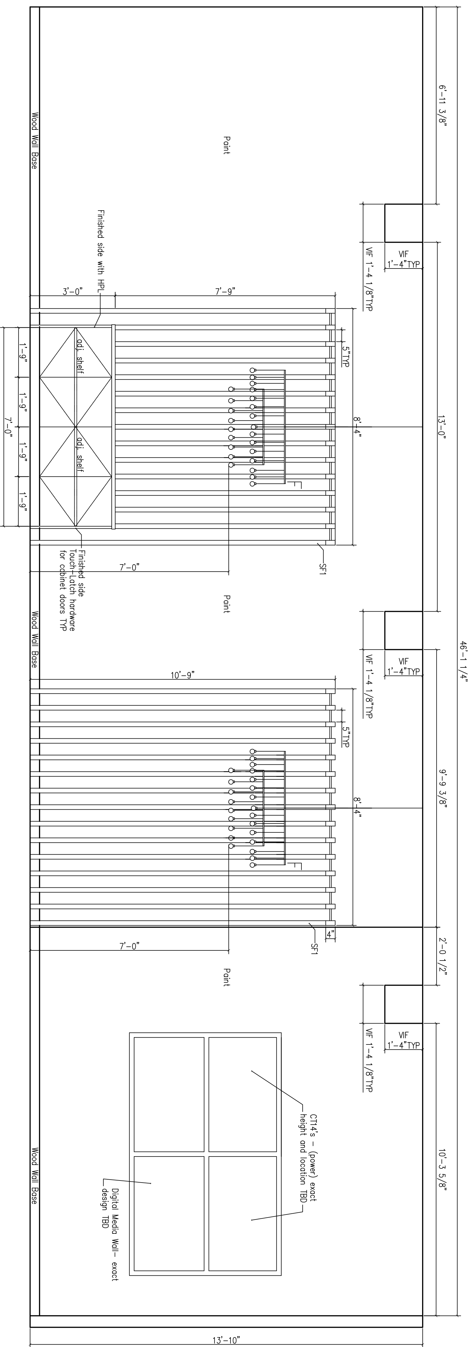
1.2 DIALOGUE AREA / WOODEN SLAT CANOPY ELEVATION 1/2" = 1'-0"
