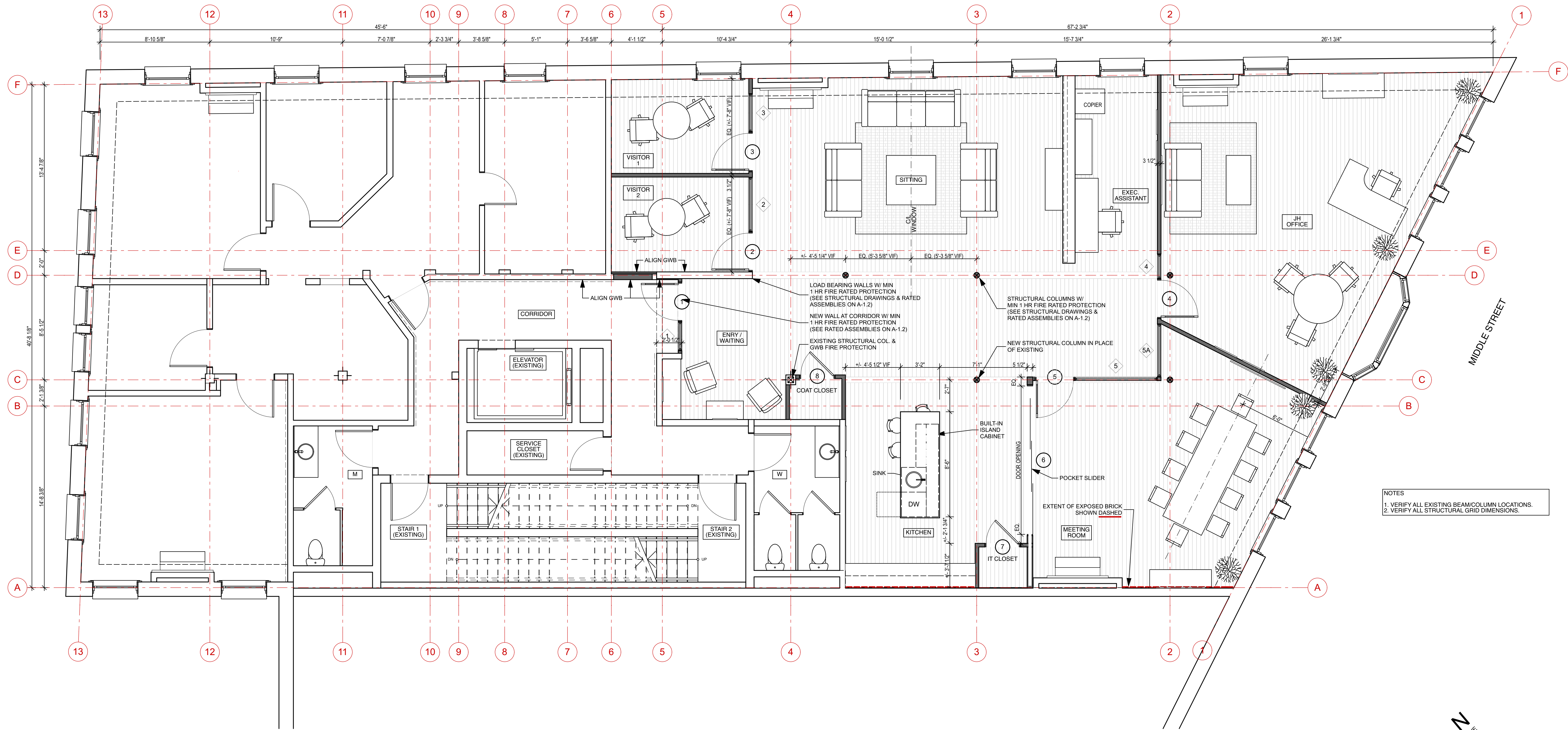
1 PROPOSED PLAN - LEVEL 2 SCALE: 1/4" = 1'-0"
