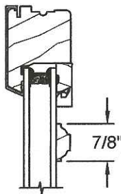
Full Surround 7/8" Wood Grille
