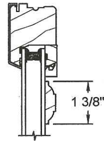
Full Surround 1 3/8" Wood Grille
