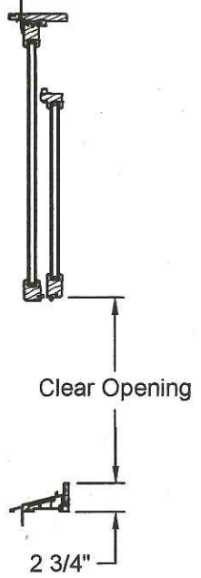
Reverse Cottage Window
