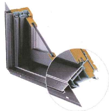
HYBRID WOOD FRAME/ CLAD SASH
