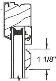
Full Surround 1 1/8" Wood Grille
