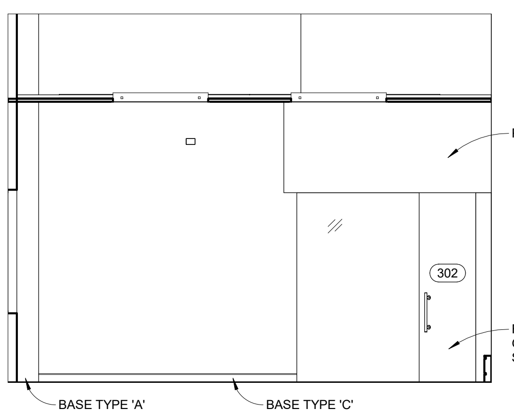
4 3RD FLOOR 302 WEST 1/4" = 1'-0"
