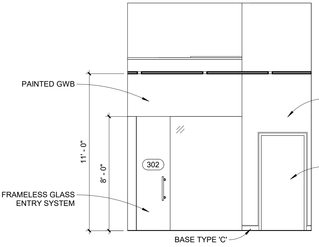
5 3RD FLOOR LOBBY EAST 1/4" = 1'-0"
