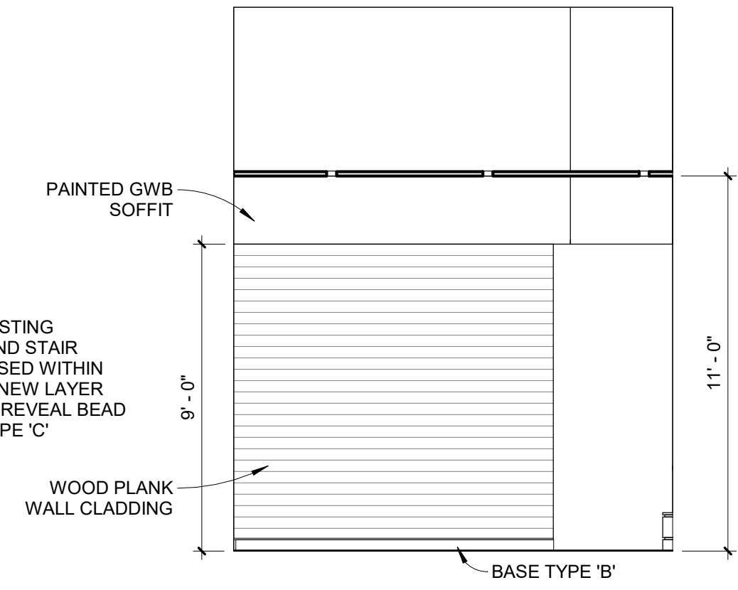
7 3RD FLOOR LOBBY WEST 1/4" = 1'-0"
