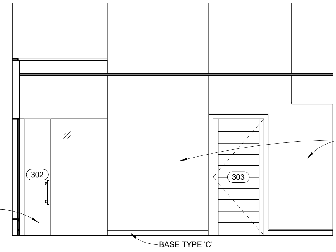
2 3RD FLOOR LOBBY SOUTH 1/4" = 1'-0"
