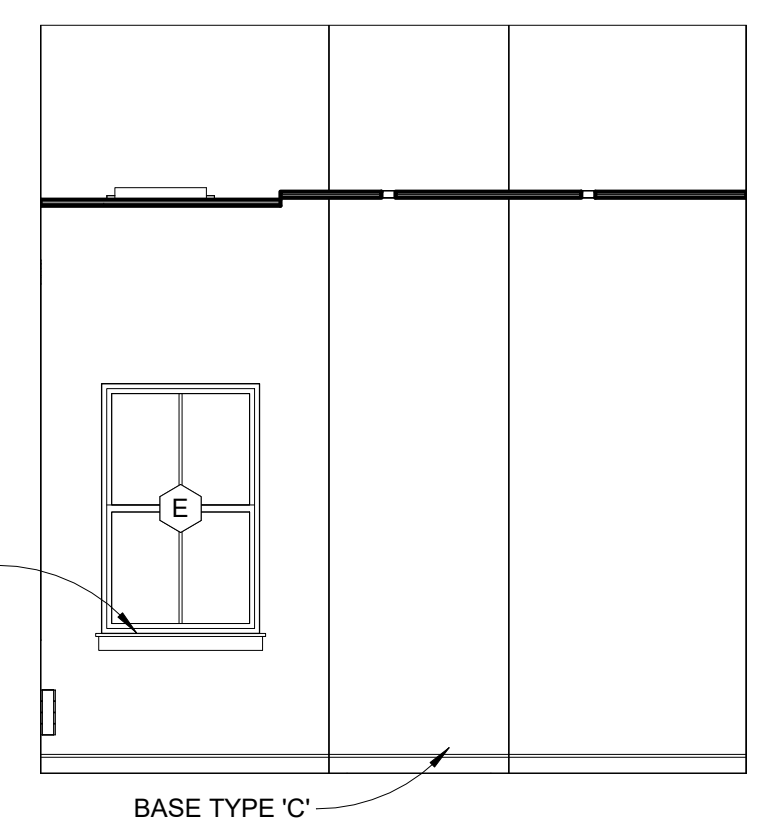
6 3RD FLOOR 302 SOUTH 1/4" = 1'-0"
