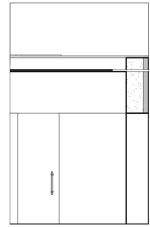
3 3RD FLOOR LOBBY ANGLED WALL 1/4" = 1'-0"
