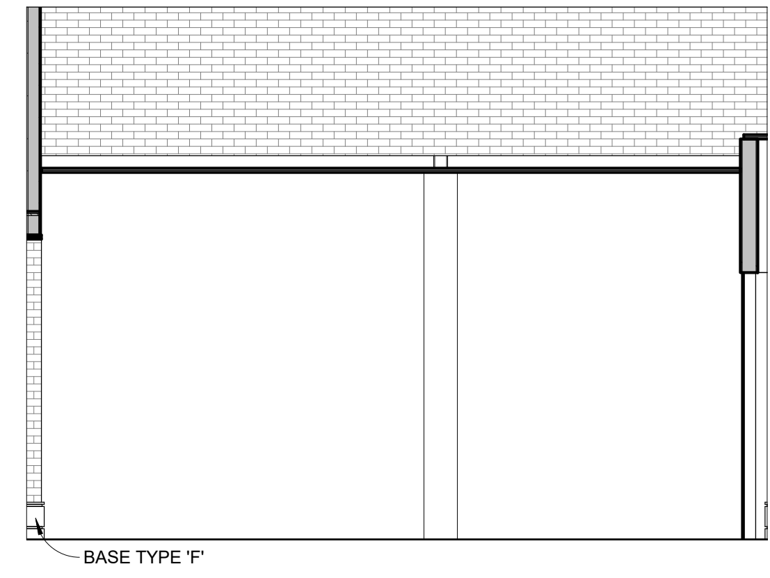
8 3RD FLOOR LOBBY NORTH 1/4" = 1'-0"
