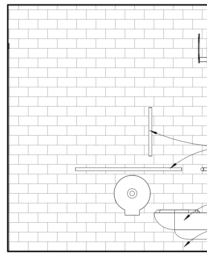
02 TOILET ELEVATION 1/2" = 1'-0"
