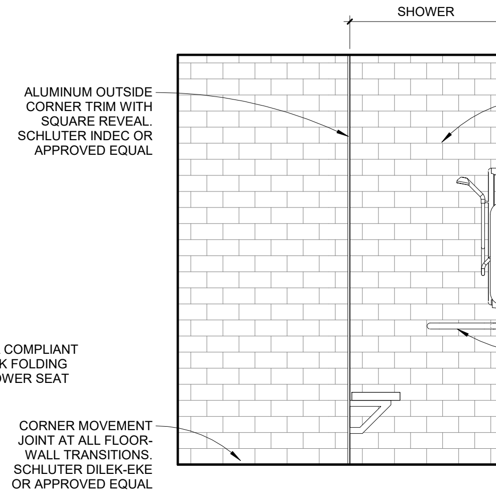
04 SHOWER ELEVATION 1/2" = 1'-0"
