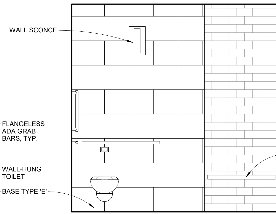
03 TOILET/SHOWER ELEVATION 1/2" = 1'-0"
