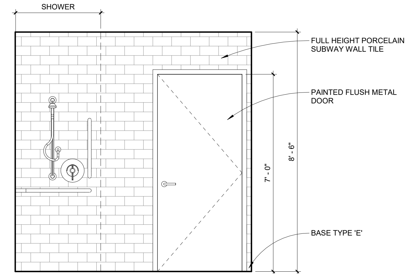
05 SHOWER ELEVATION 1/2" = 1'-0"
