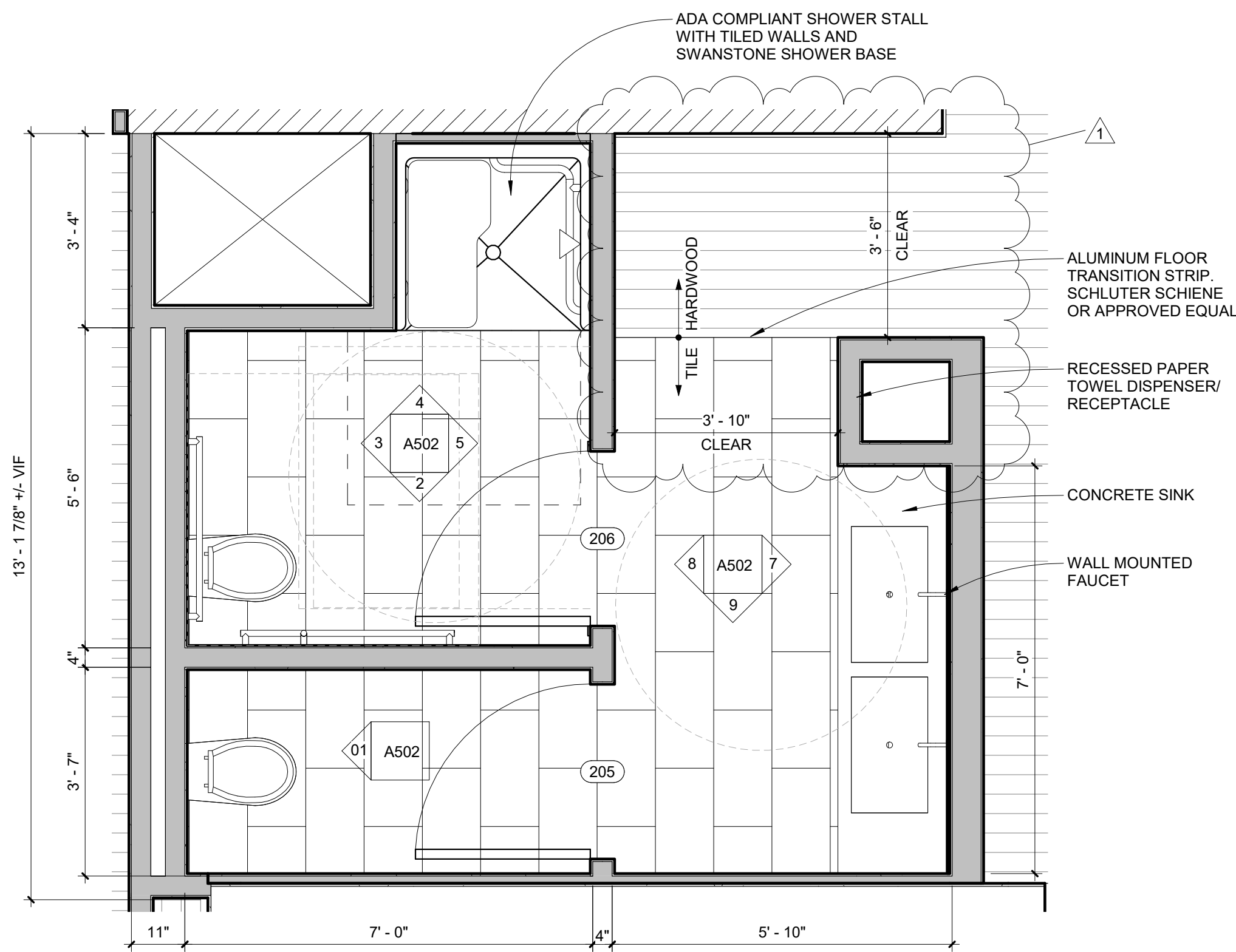
06 TYPICAL BATHROOM ENLARGED PLAN 1/2" = 1'-0"
