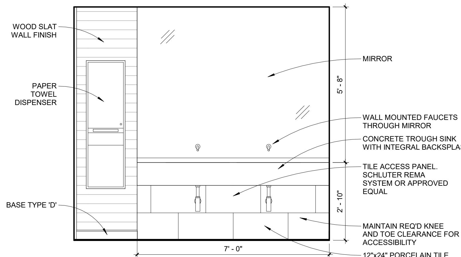
07 BATHROOM SINK ELEVATION 1/2" = 1'-0"
