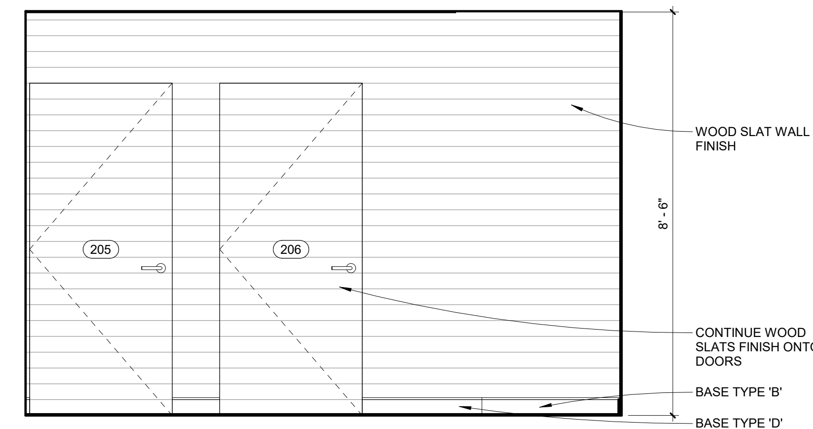
08 BATHROOM STALL DOORS ELEVATION 1/2" = 1'-0"
