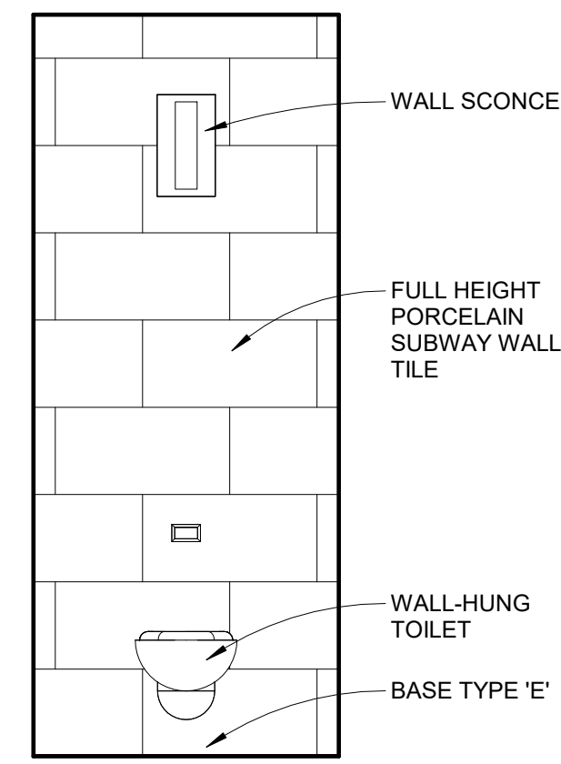
01 TOILET ELEVATION 1/2" = 1'-0"
