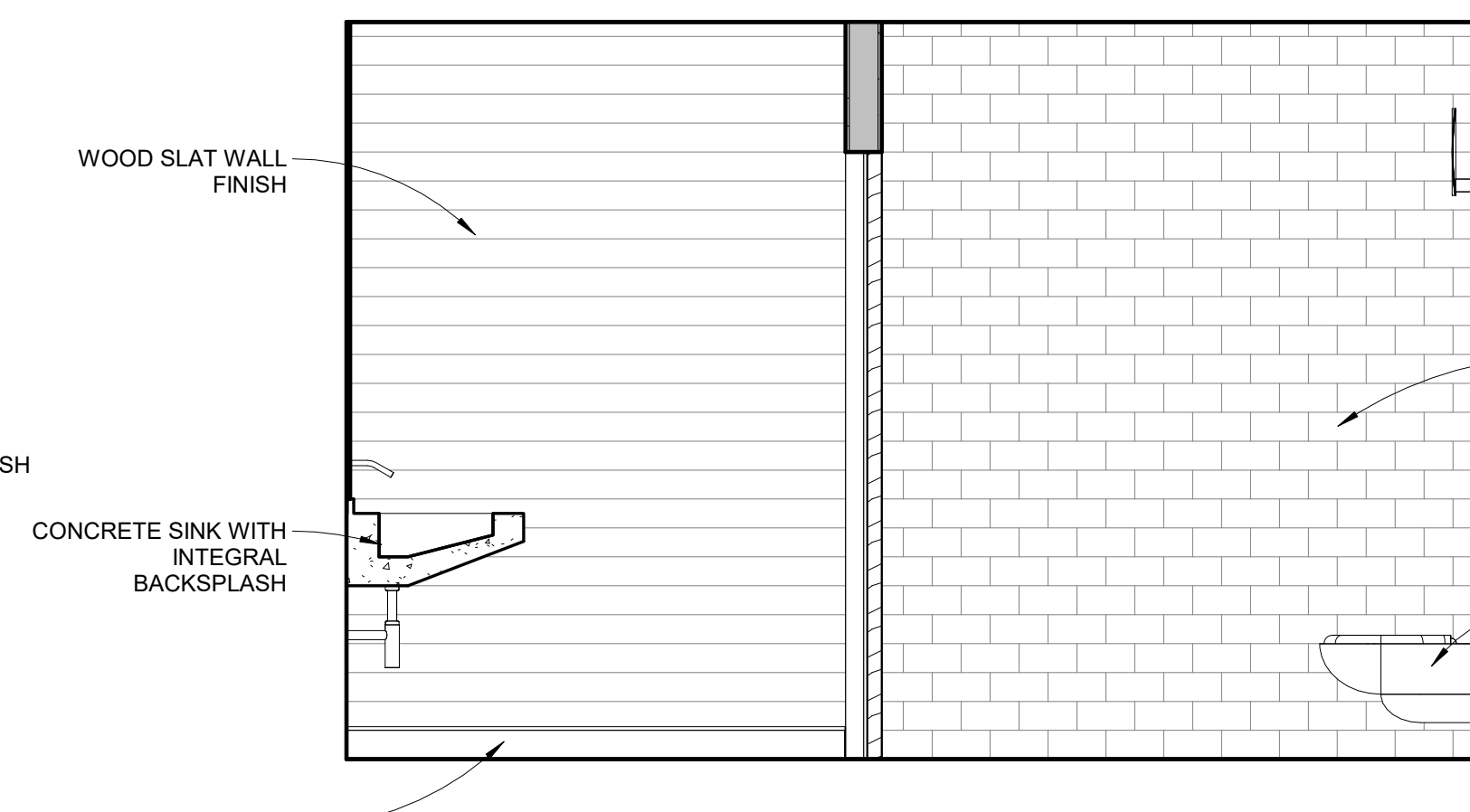
09 TOILET ELEVATION 1/2" = 1'-0"
