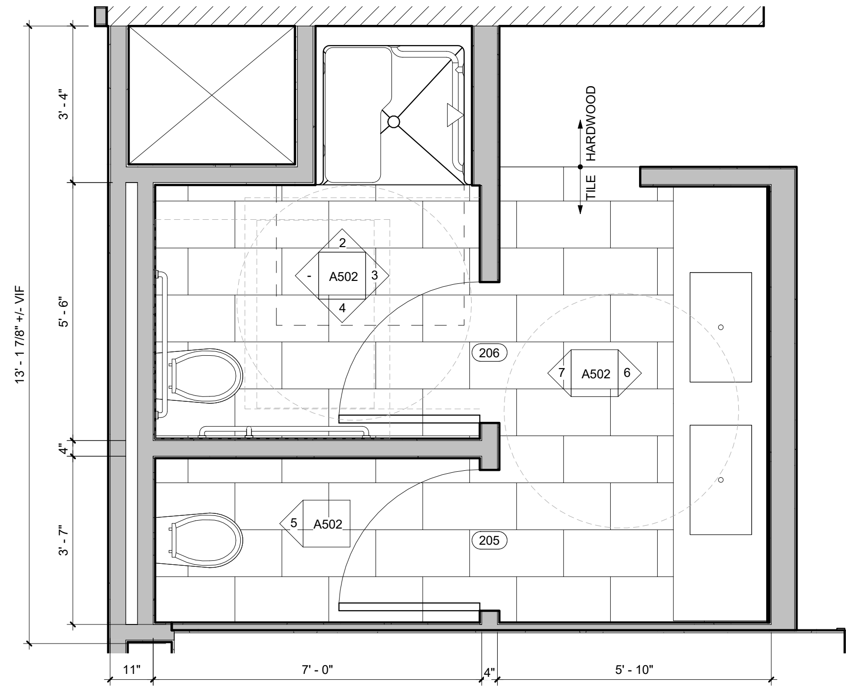
1 TYPICAL BATHROOM ENLARGED PLAN 1/2" = 1'-0"
