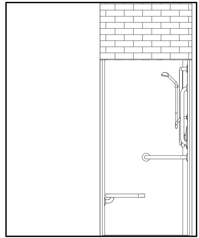
2 SHOWER ELEVATION 1/2" = 1'-0"
