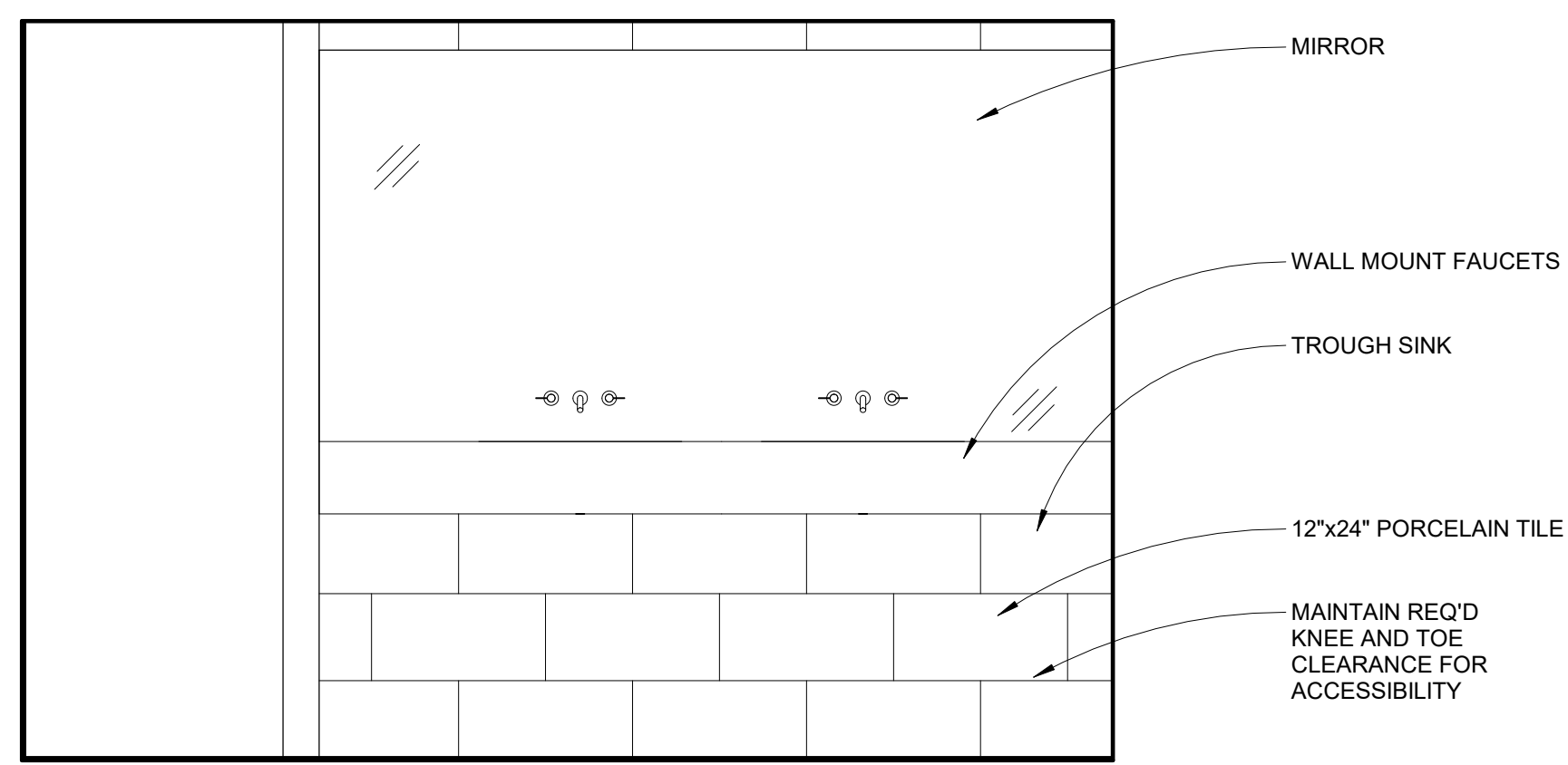
6 BATHROOM SINK ELEVATION 1/2" = 1'-0"
