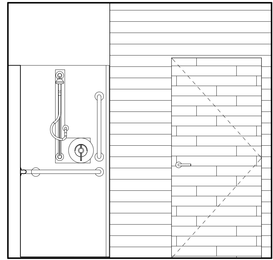
3 SHOWER FIXTURE ELEVATION 1/2" = 1'-0"
