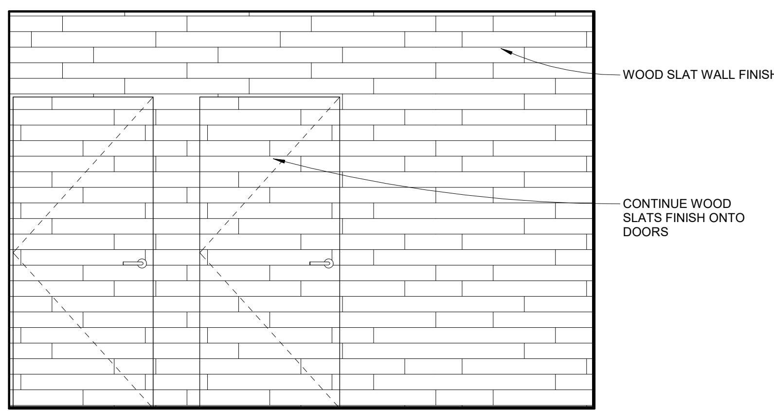
7 BATHROOM STALL DOORS ELEVATION 1/2" = 1'-0"
