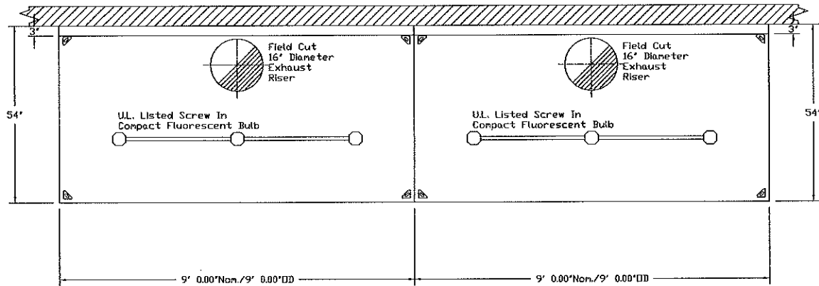
PLAN VIEW - Hood #1 9' 0.00" LONG 5424EX-2
