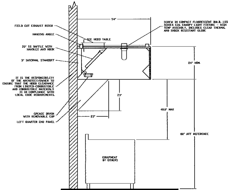
SECTION VIEW - MODEL 5424EX-2 HOOD -- #1
