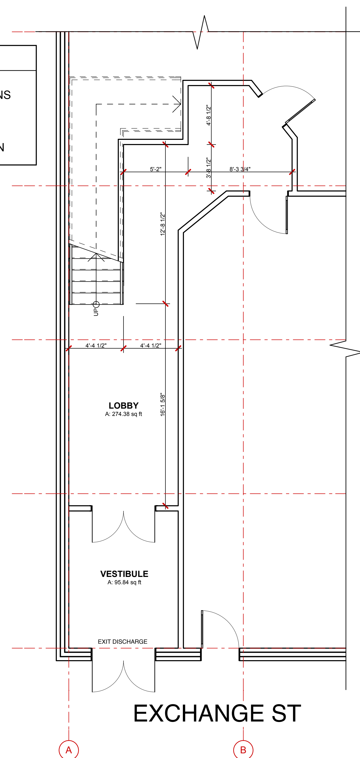
2 STREET LEVEL: EXISTING CONDITIONS SCALE: 1/4" = 1'-0"
