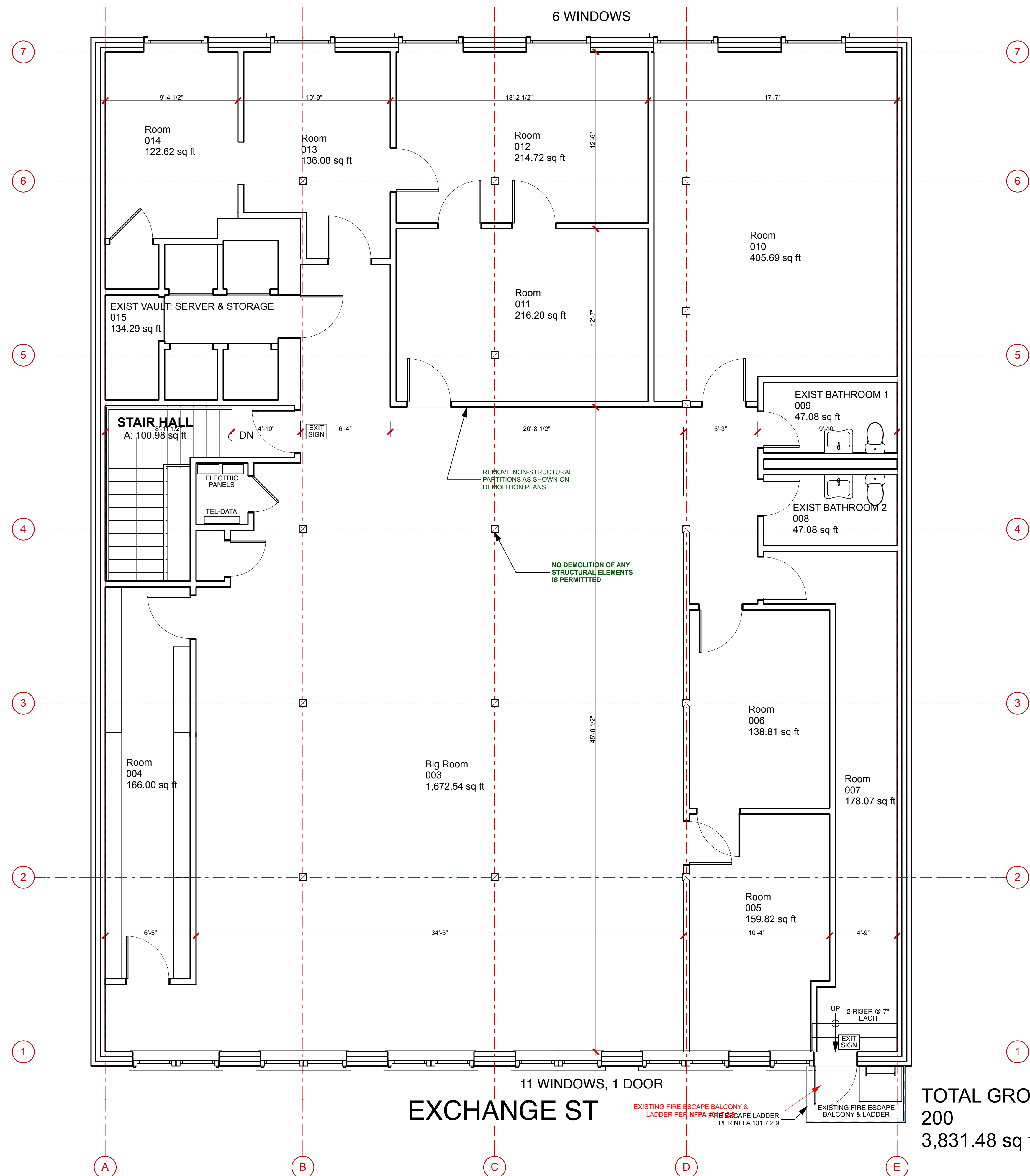
1 UPPER LEVEL: EXISTING CONDITIONS SCALE: 1/4" = 1'-0"
