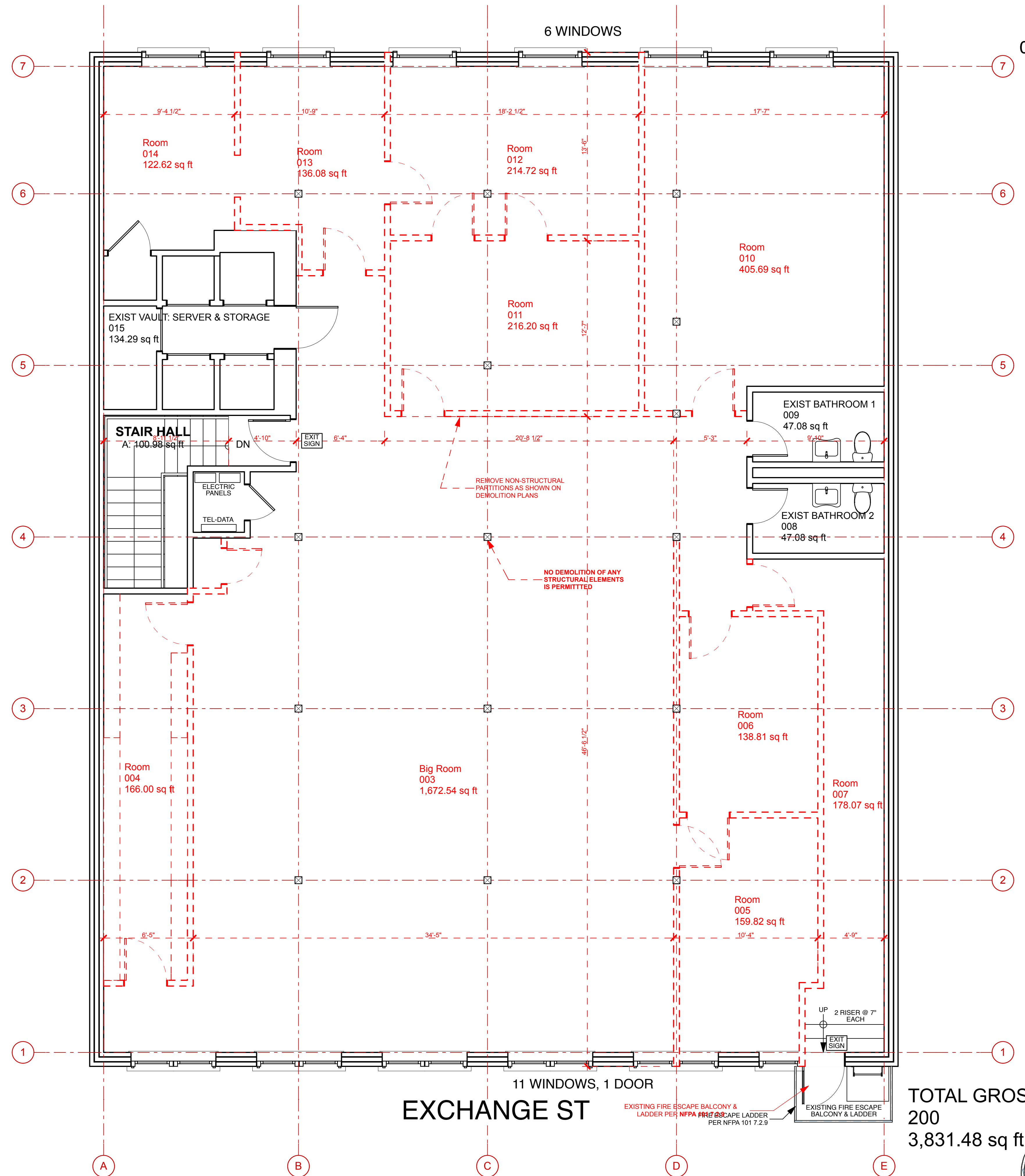
1 2ND FLOOR LEVEL SCALE: 1/4" = 1'-0"
