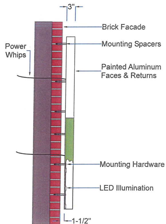
M1 Mounting Detail View
