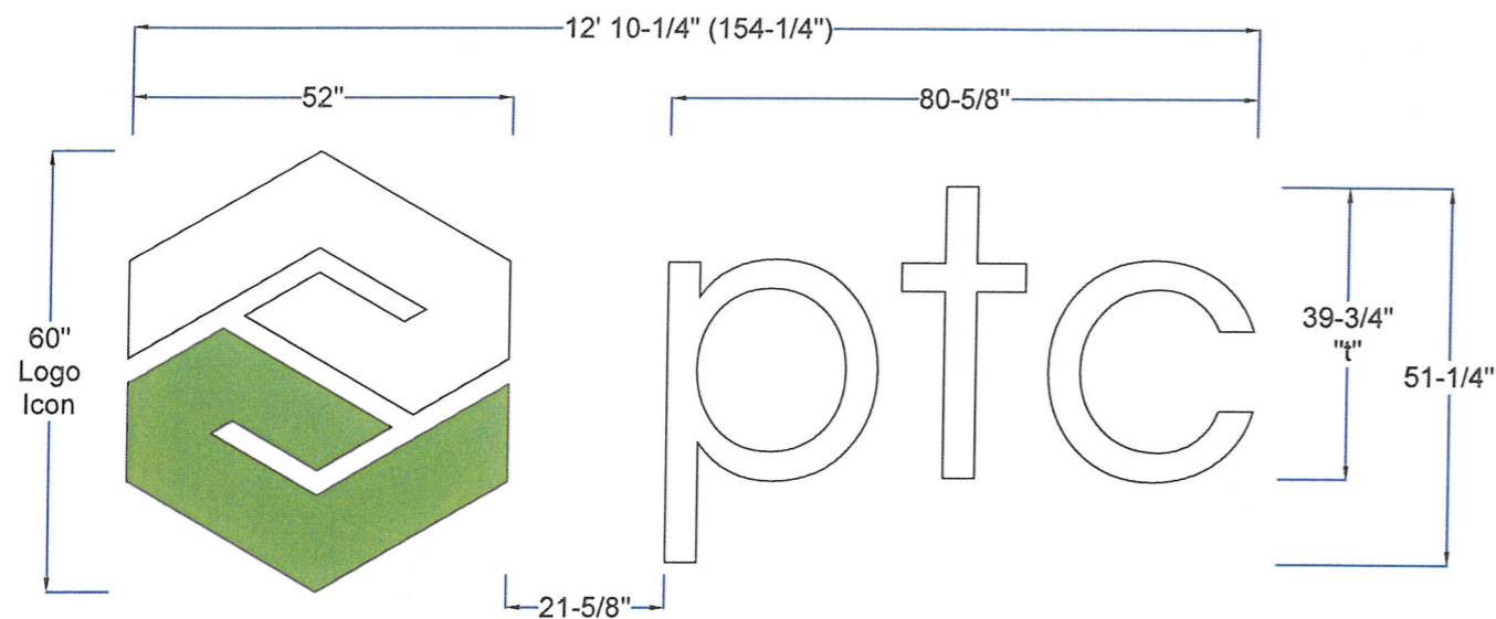
E1 Elevation: (Qty: 1) #8692 Halo Illuminating Channel Letters 60" x 154-1/4" = 64.2 Sq. Ft.
