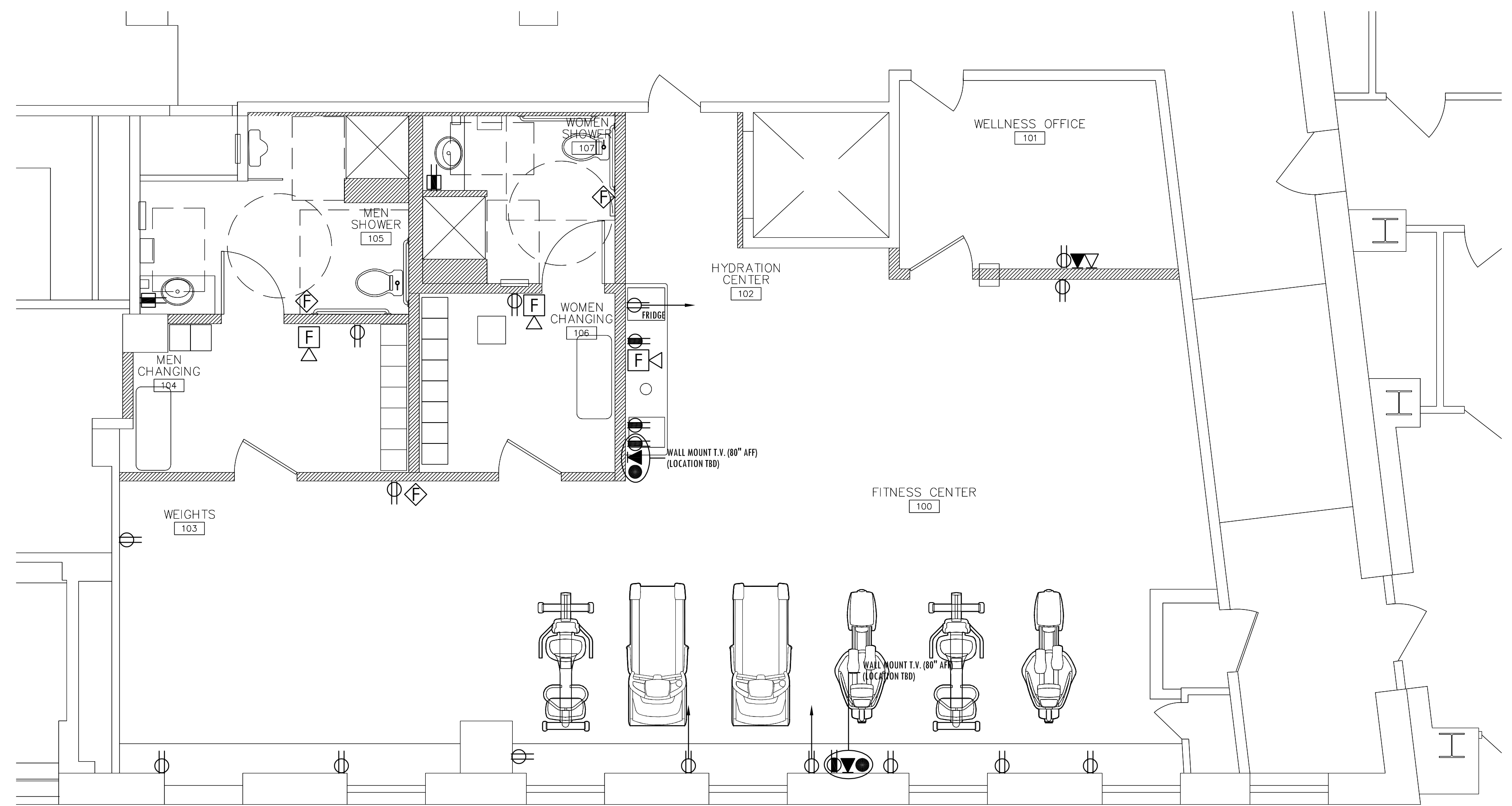
1ST FLOOR FITNESS CENTER - LIGHTING & EMERGENCY LIGHTING LAYOUT
