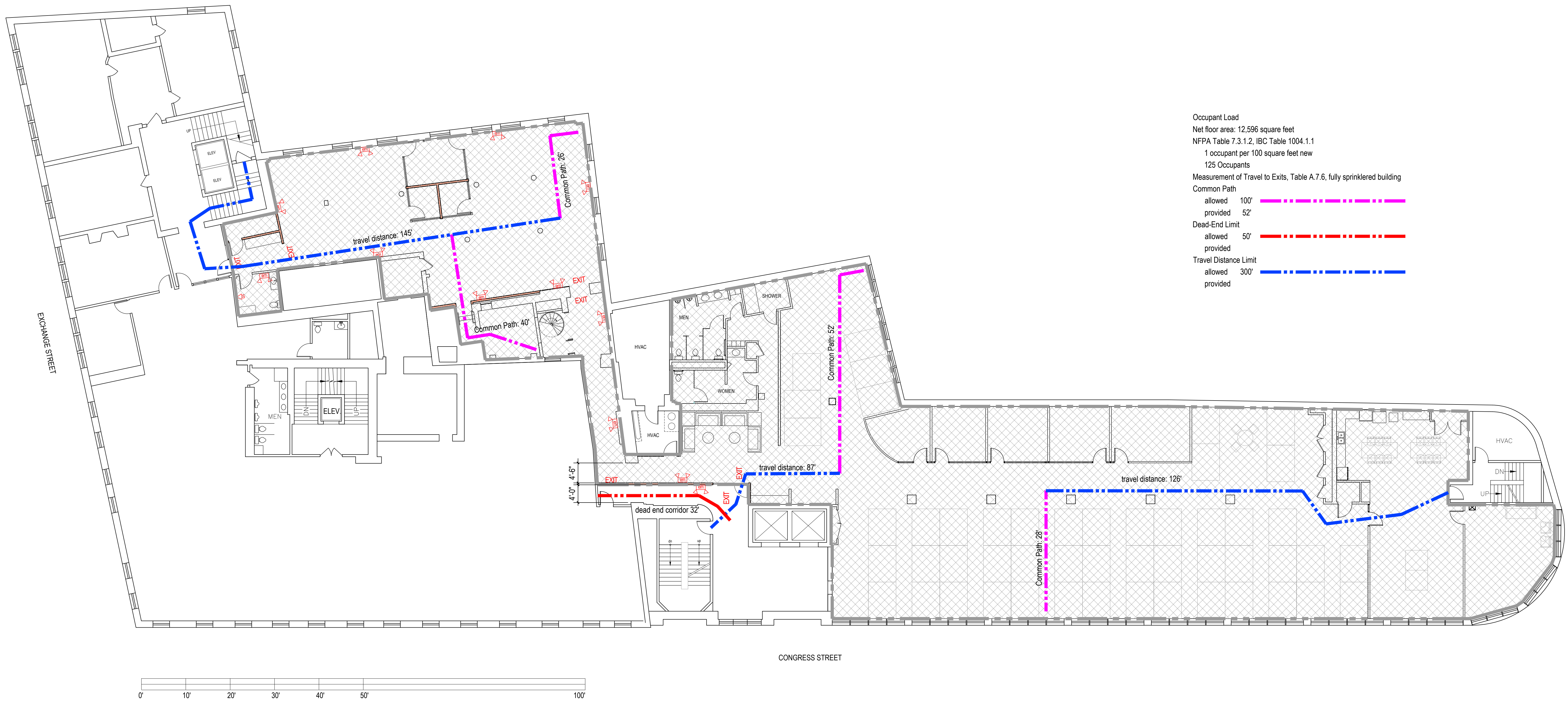
1 3rd Floor Plan, Life Safety Plan 3/32"= 1'-0"
