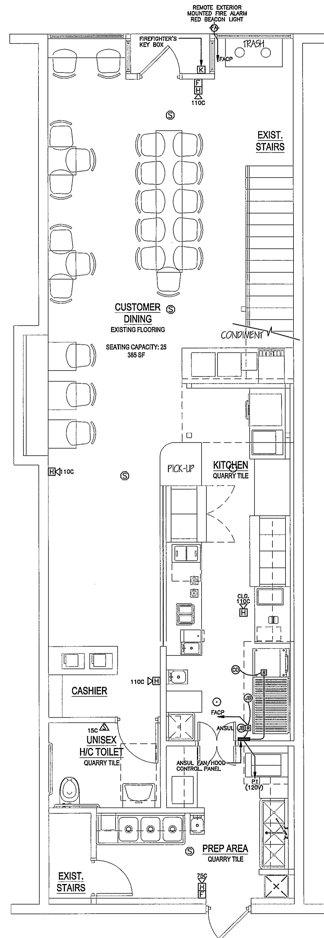
FIRST FLOOR PLAN- FIRE ALARM Scale: 1/4"=1'-0"
