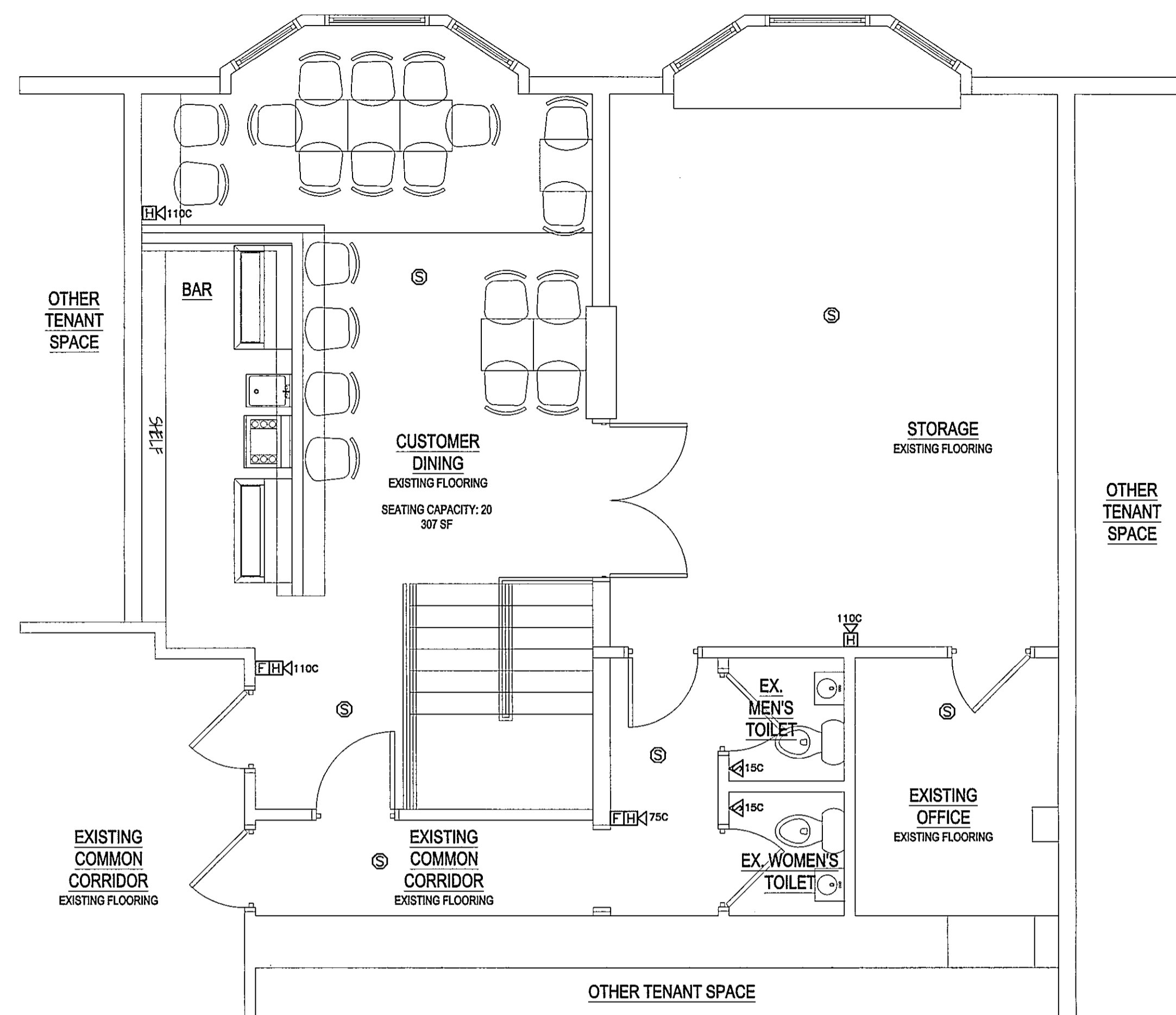
SECOND FLOOR PLAN- FIRE ALARM Scale: 1/4"=1'-0"
