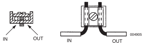
CORRECT – SEPARATE INCOMING AND OUTGOING CONDUCTORS
