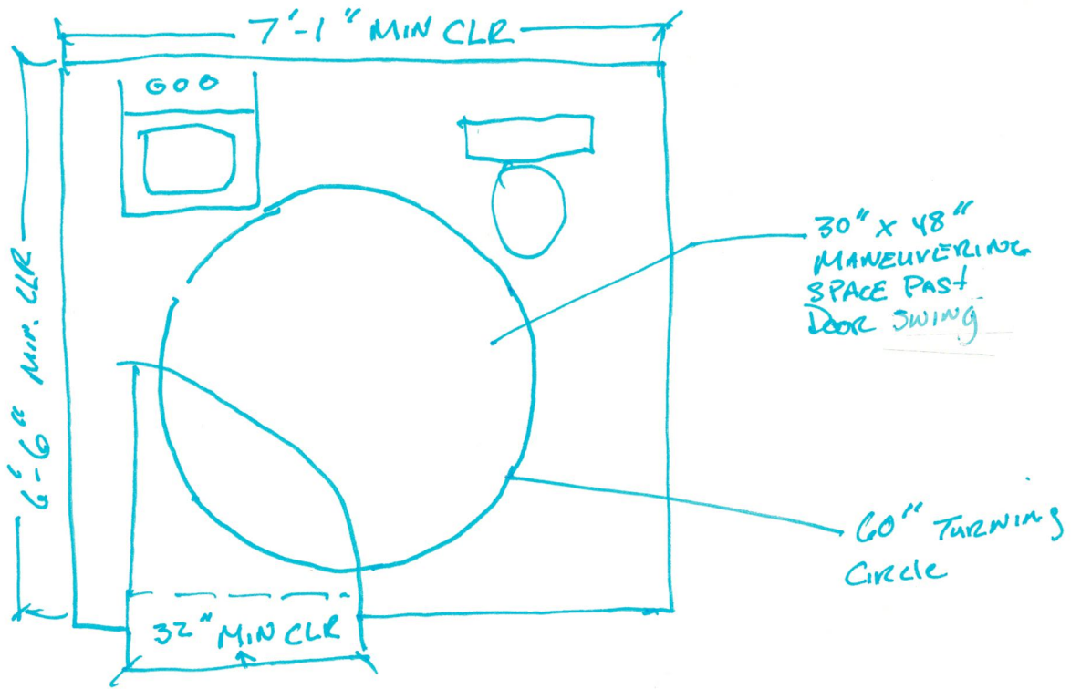
NEW BATH ROOM PLAN
