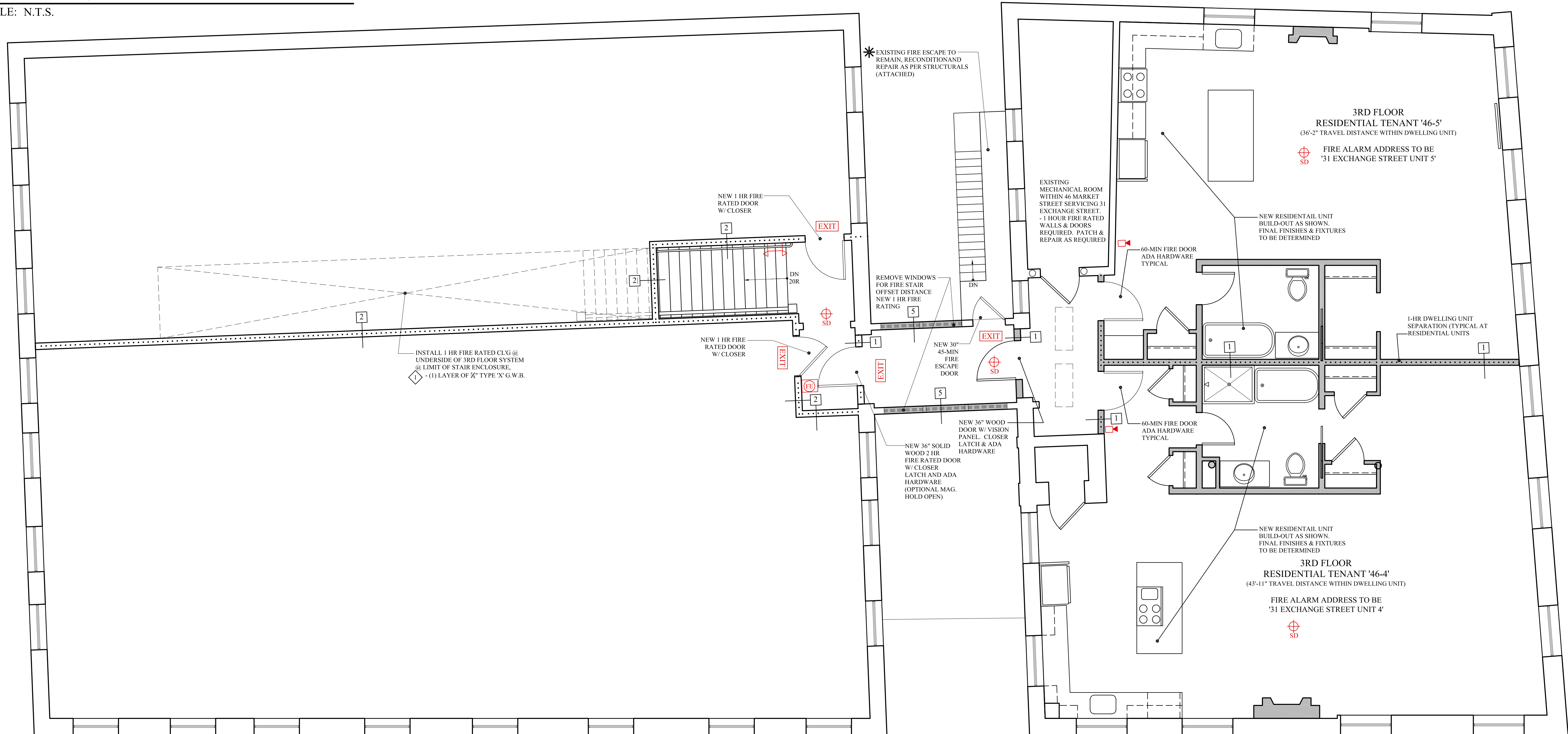
THIRD FLOOR PLAN SCALE: 1/4" = 1'-0"
