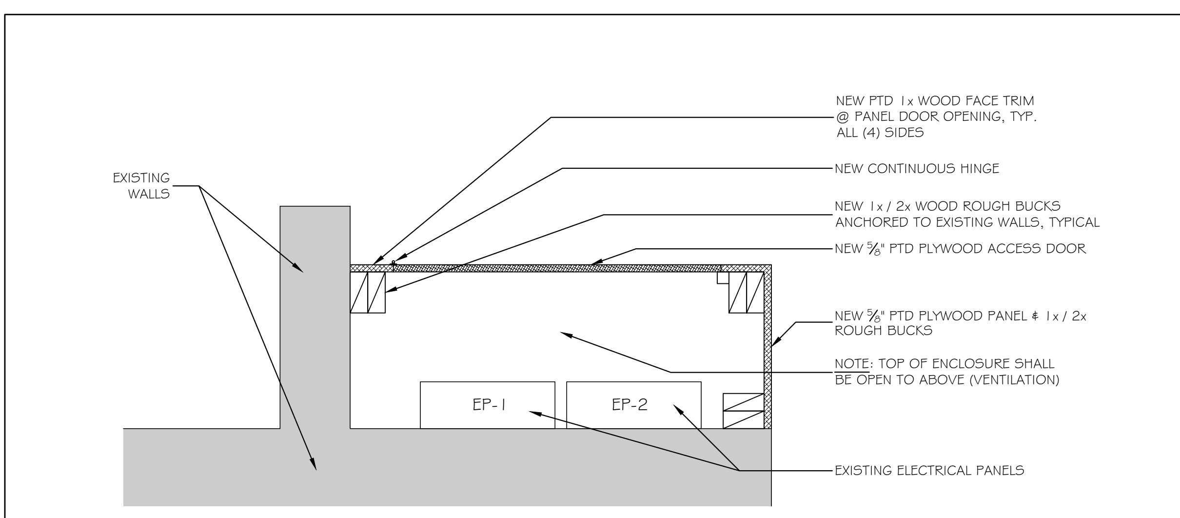
⑤ ELECTRICAL PANEL DECORATIVE ACCESS PANEL DETAIL 3" = 1'-0"
