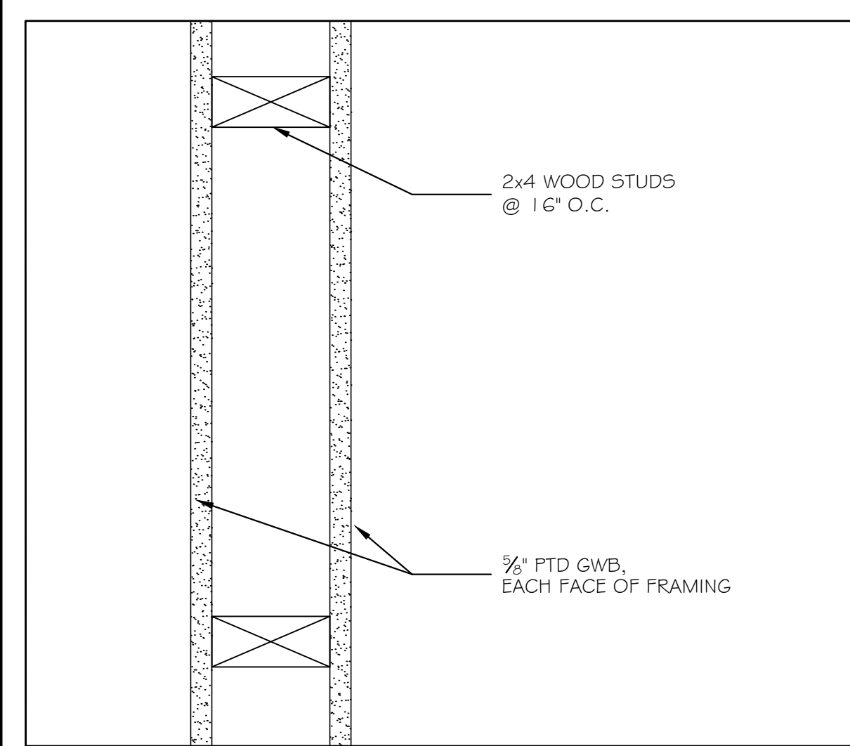
① TYPICAL PARTITION TYPE 3" = 1'-0"
