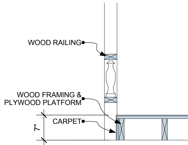
DETAIL scale: 3/4"=1'
