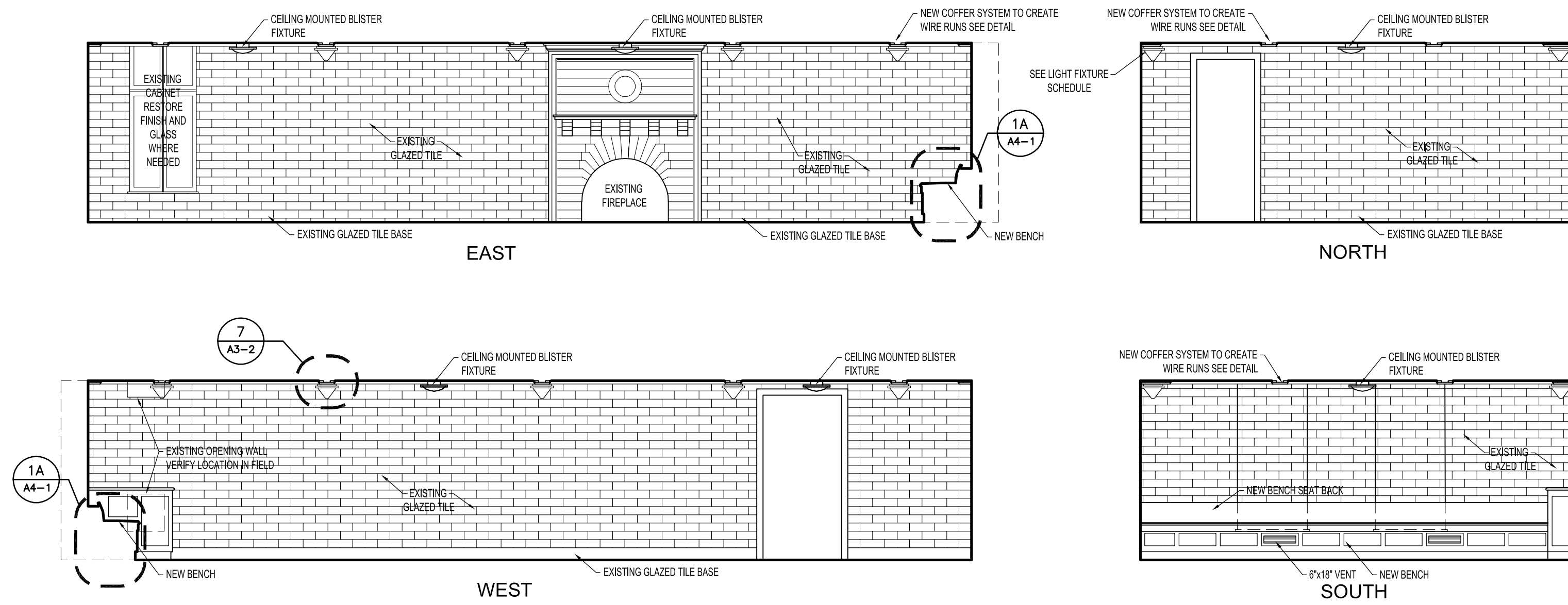
1 FUNCTION ROOM - 118 INTERIOR ELEVATIONS A2-4 1/4" = 1'-0"
