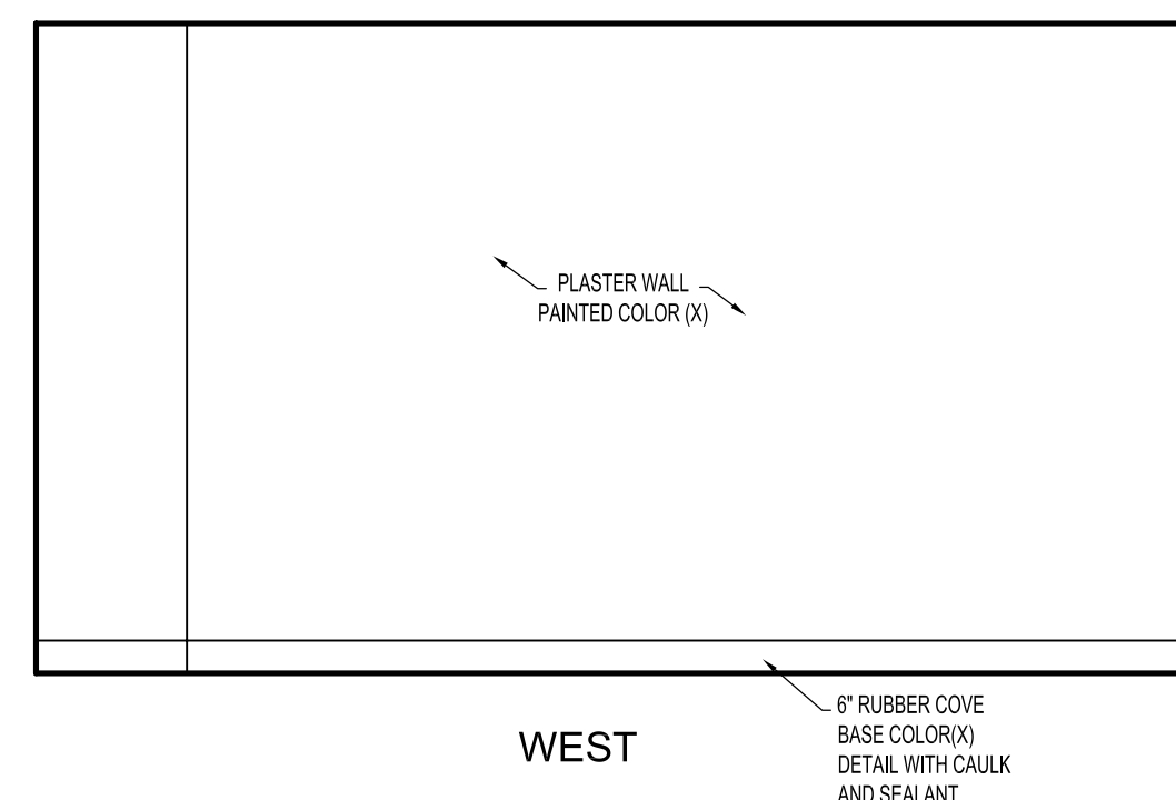
4 DISHROOM - 110 INTERIOR ELEVATIONS A2-3 1/4" = 1'-0"
