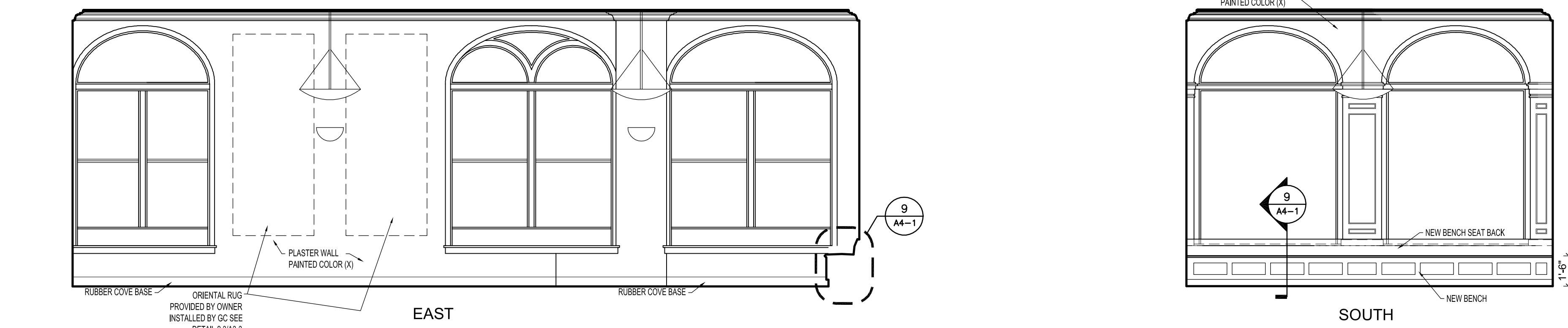
2 SOUTH DINING ROOM - 105 INTERIOR ELEVATIONS A2-2 1/4" = 1'-0"
