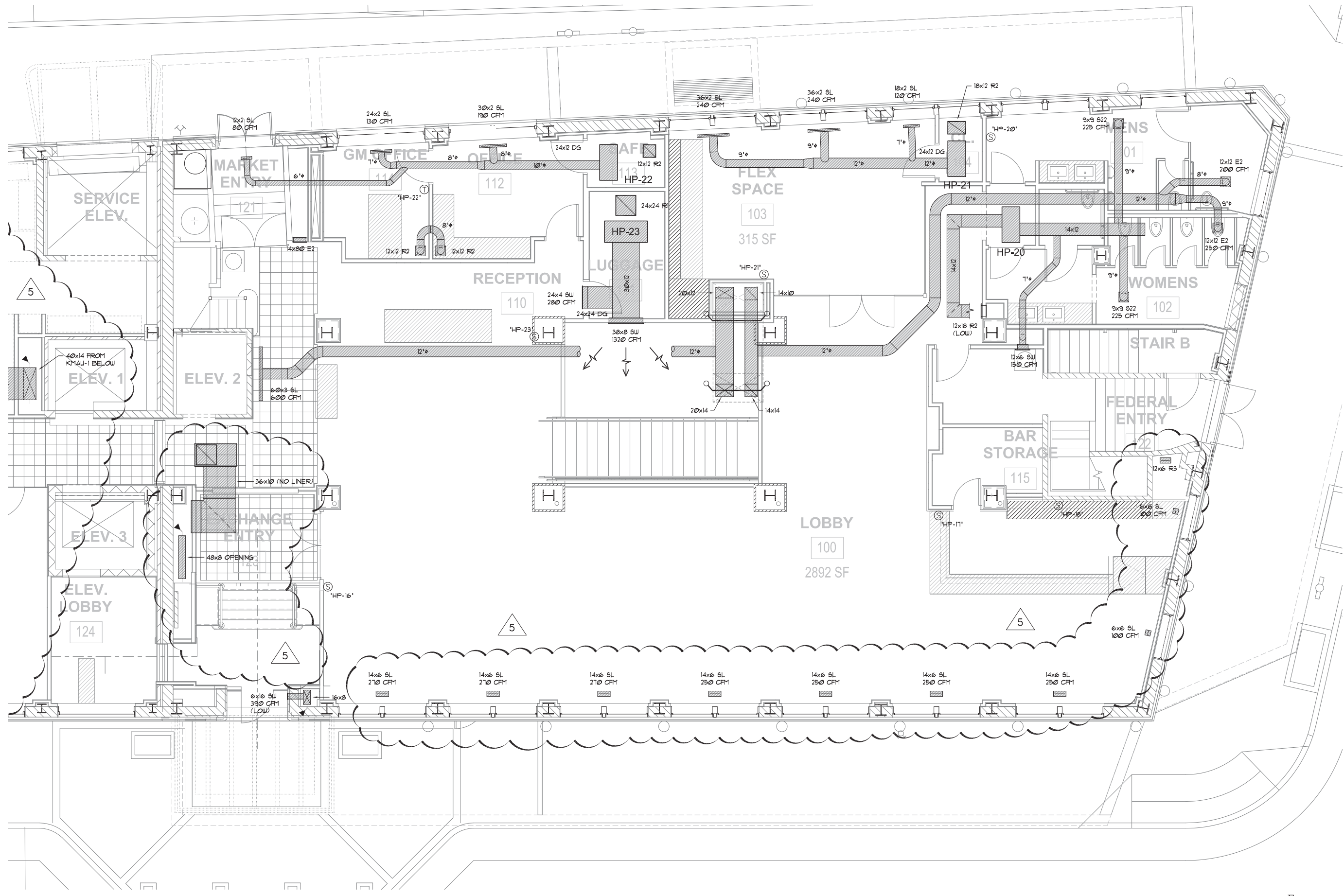
ENLARGED FIRST FLOOR PLAN - HVAC SCALE: 1/4"=1'-0"
