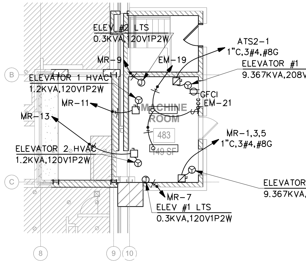
2 | ELEVATOR MACHINE ROOM ELECTRICAL PLAN SCALE: 1/8"=1'-0"
