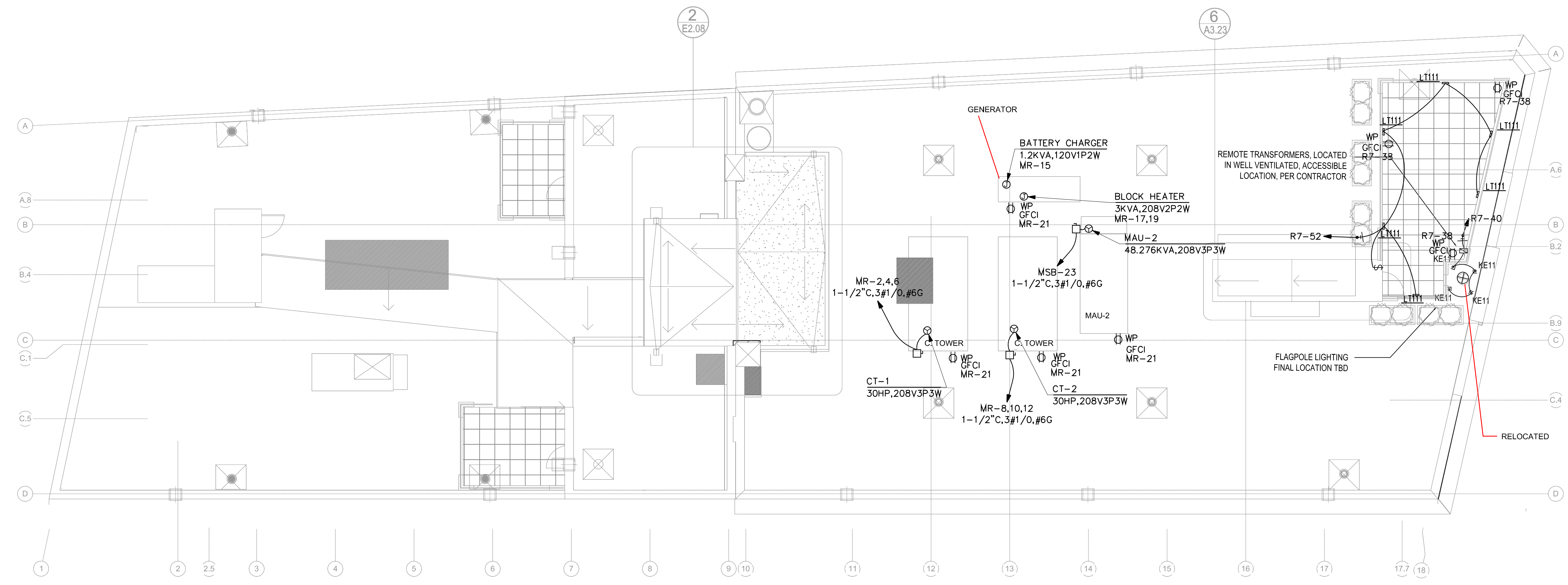
2 | ELEVATOR MACHINE ROOM ELECTRICAL PLAN SCALE: 1/8"=1'-0"
