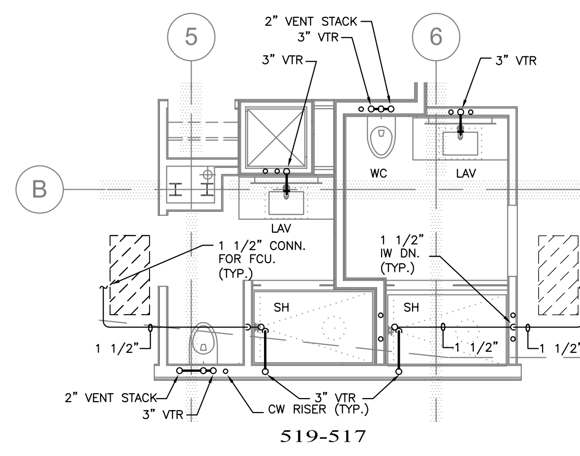
2 TYPICAL UNITS - PLUMBING SCALE: 1/4"=1'-0"
