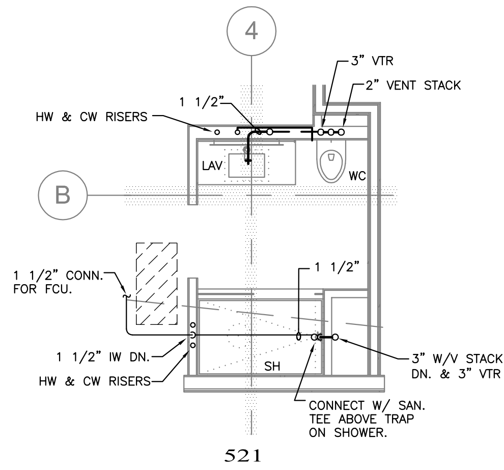
1 TYPICAL UNITS - PLUMBING SCALE: 1/4"=1'-0"
