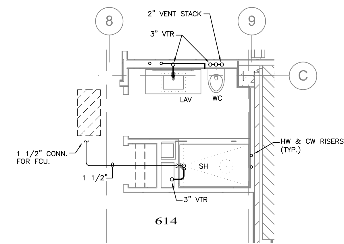
4 TYPICAL UNITS - PLUMBING SCALE: 1/4"=1'-0"
