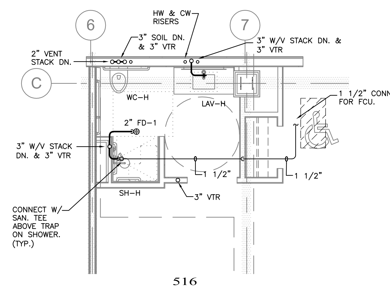
3 TYPICAL UNITS - PLUMBING SCALE: 1/4"=1'-0"
