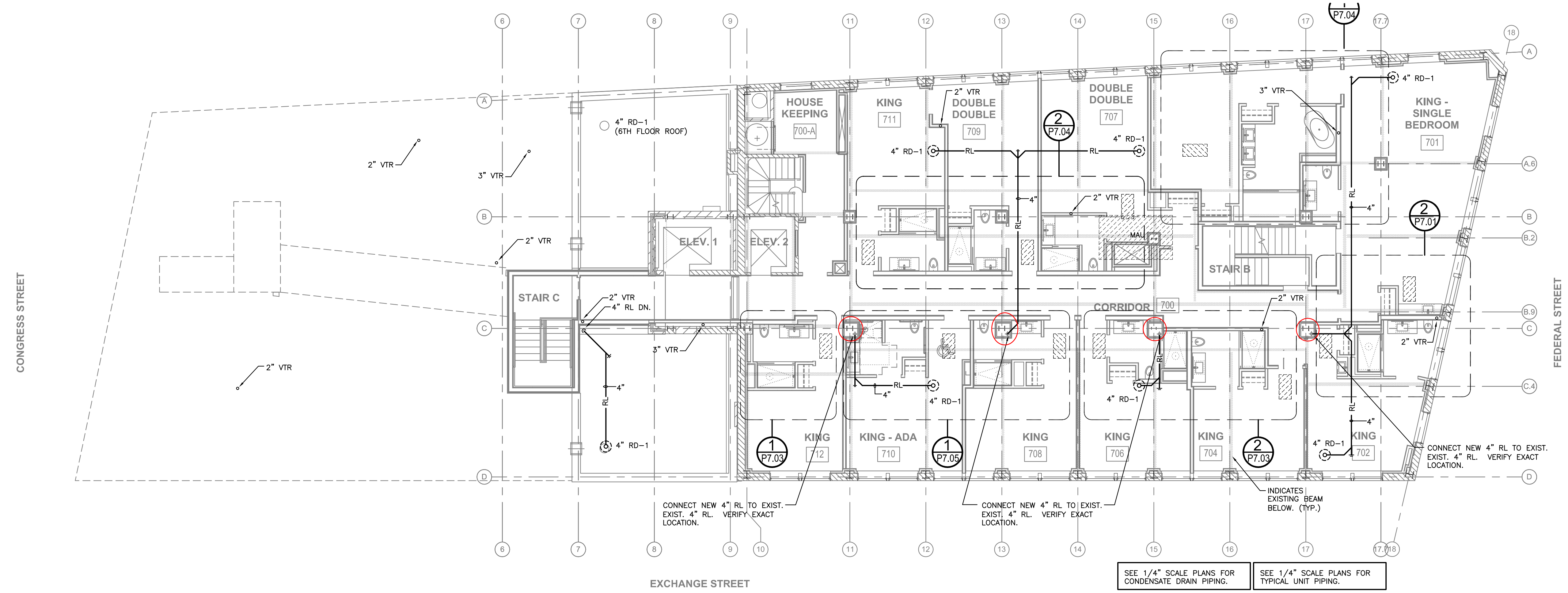
2 SEVENTH FLOOR PLAN - WASTE, VENT AND RAIN LEADER SCALE: 1/8"=1'-0"
