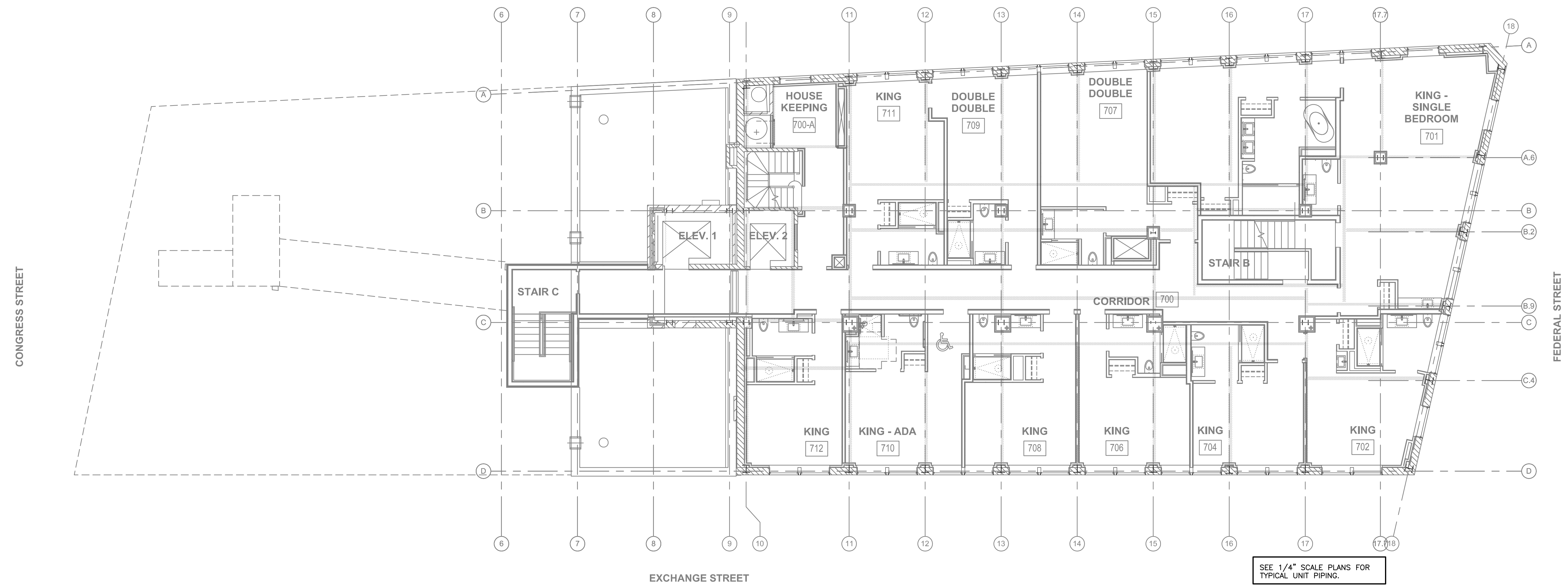
1 SEVENTH FLOOR PLAN - WATER SCALE: 1/8"=1'-0"
