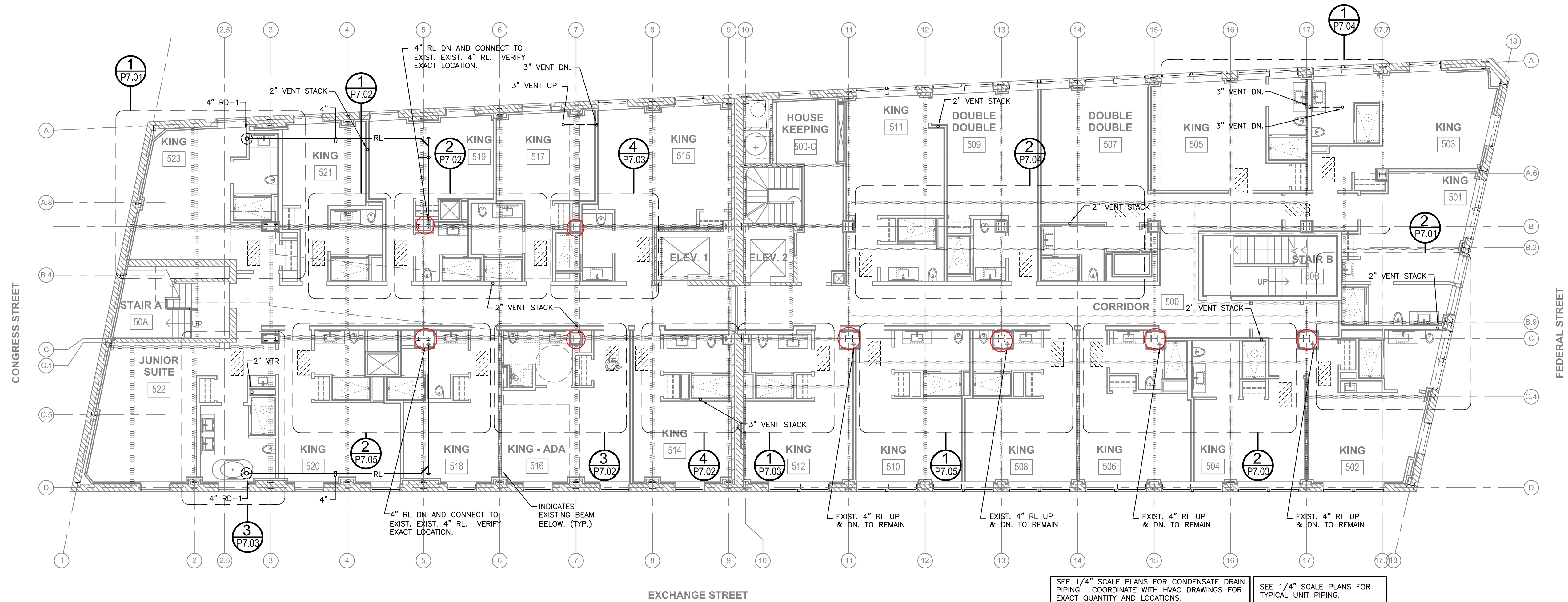
2 FIFTH FLOOR PLAN - WASTE, VENT AND RAIN LEADER SCALE: 1/8"=1'-0"
