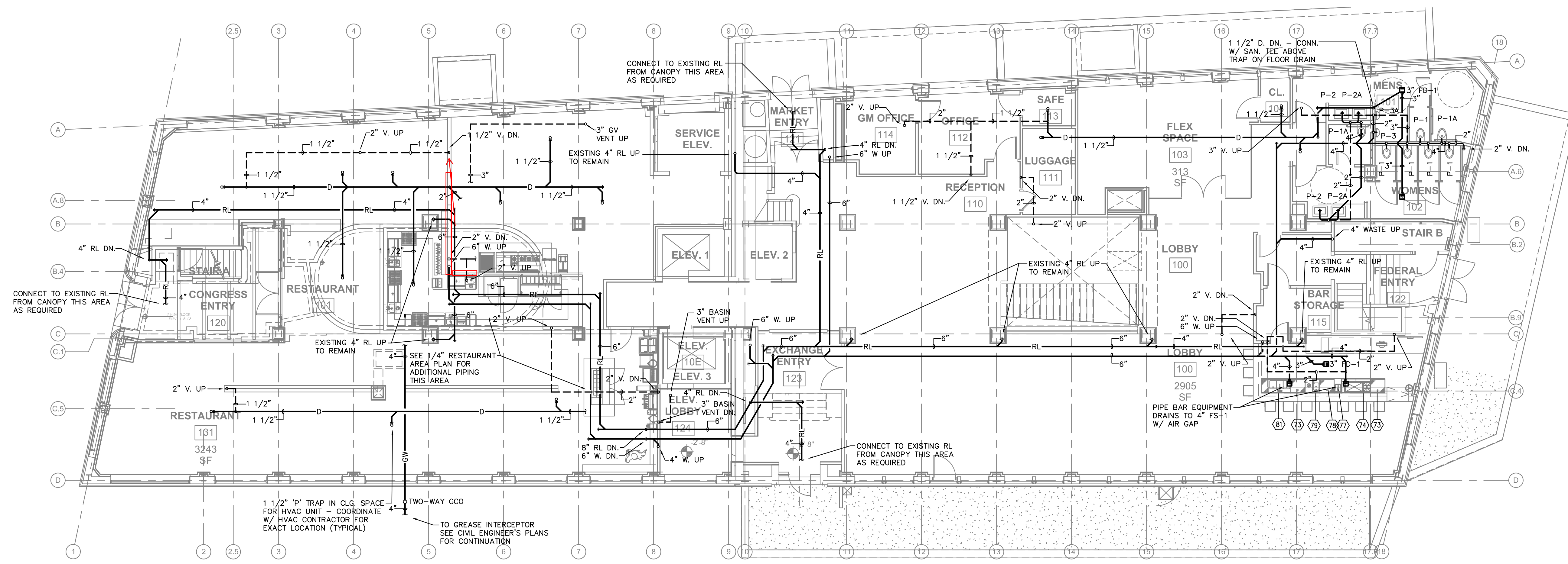
1 FIRST FLOOR PLAN - WATER SCALE: 1/8"=1'-0"
