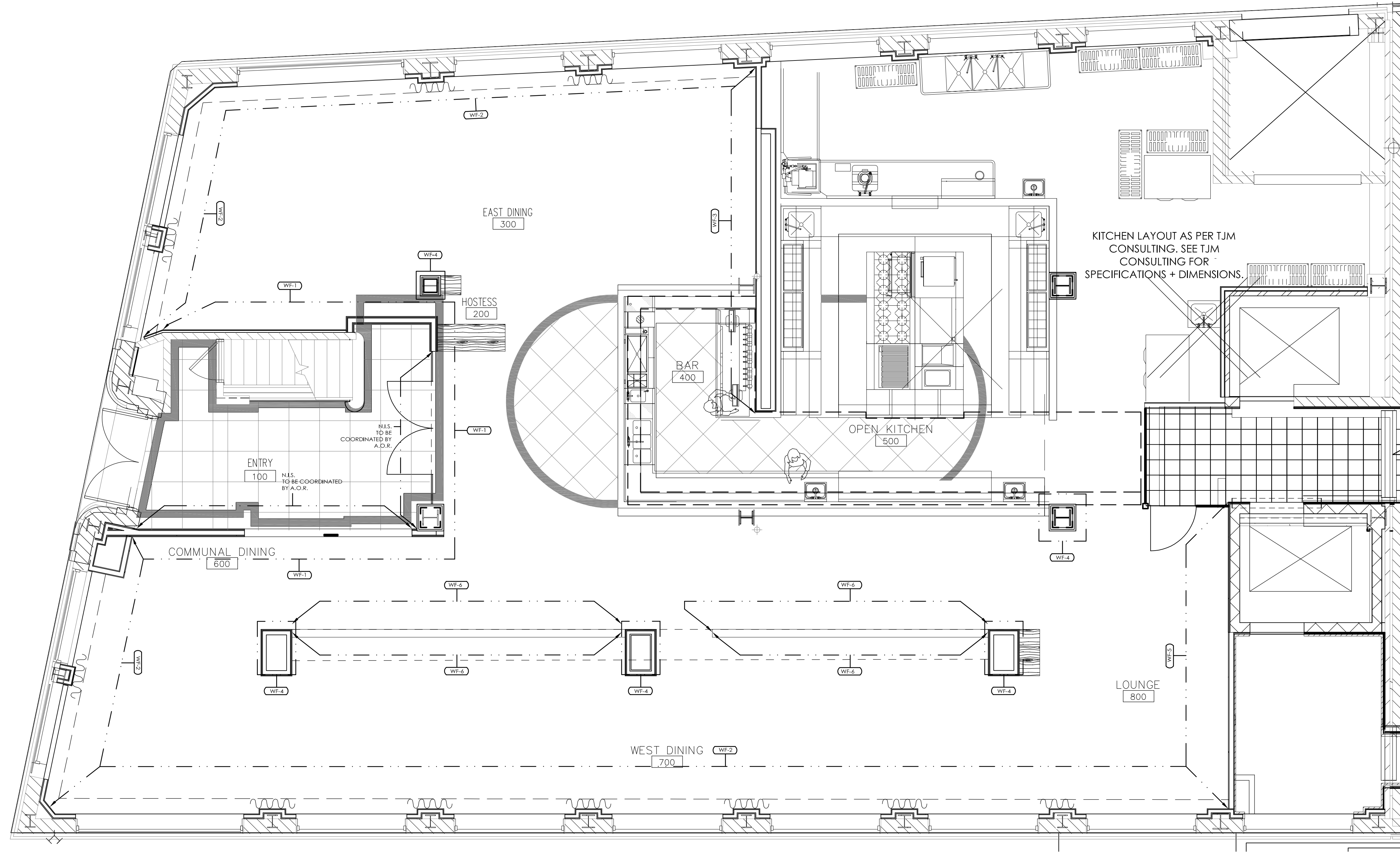
1 WALL FINISH PLAN 1/4" = 1'-0"
