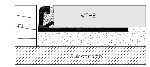
2 TRANSITION DETAIL 1'0" = 1'-0"
