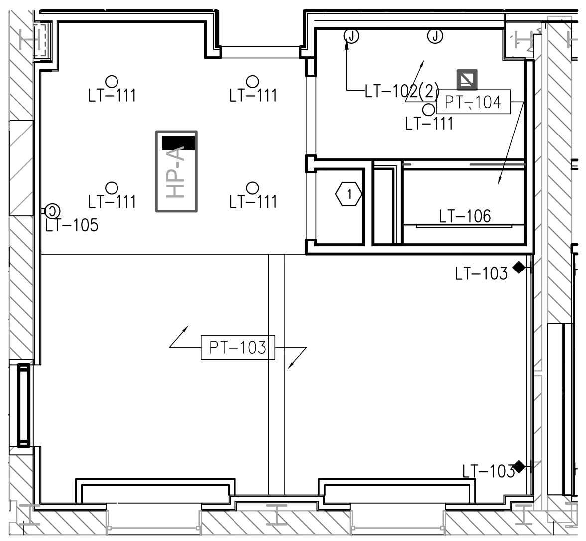
21 ROOM TYPE O REFLECTED CEILING PLAN 1/4" = 1'-0"
