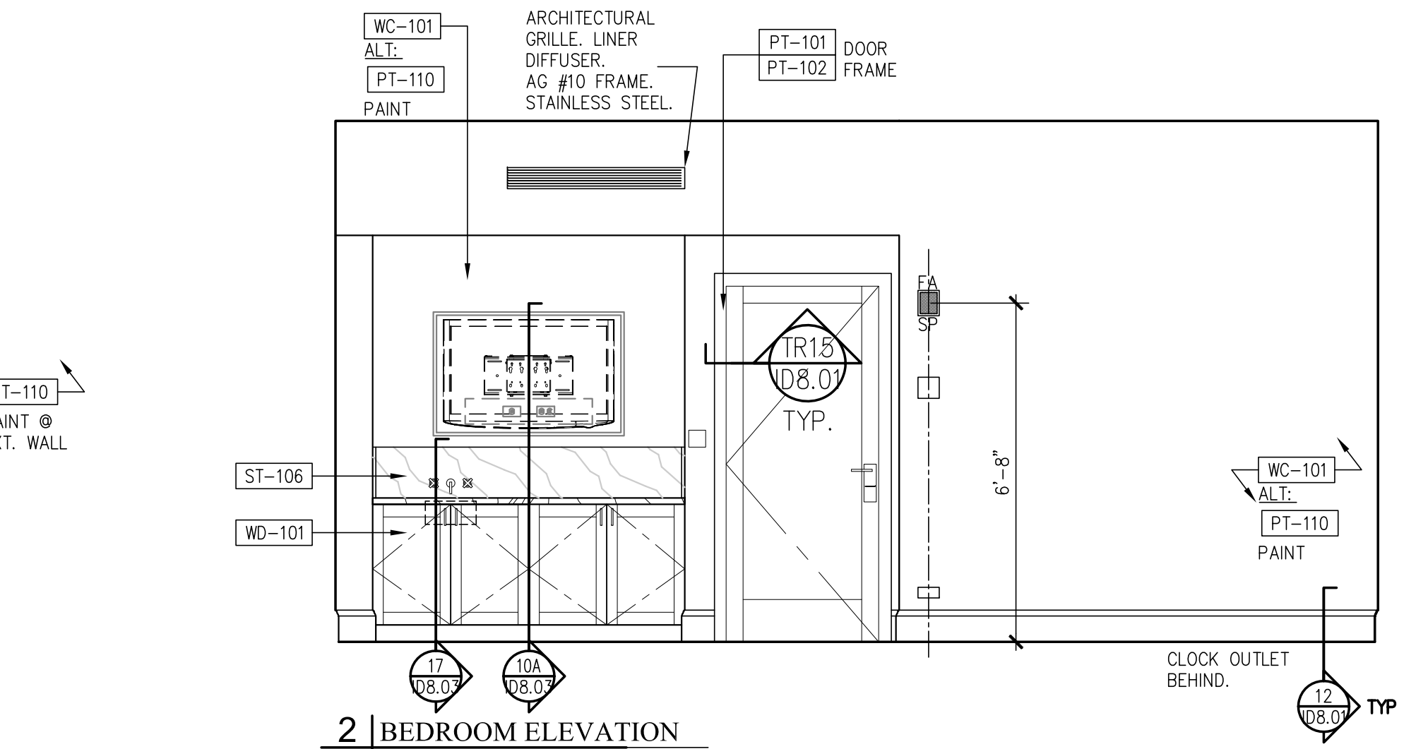
2 BEDROOM ELEVATION 3/8" = 1'-0"
