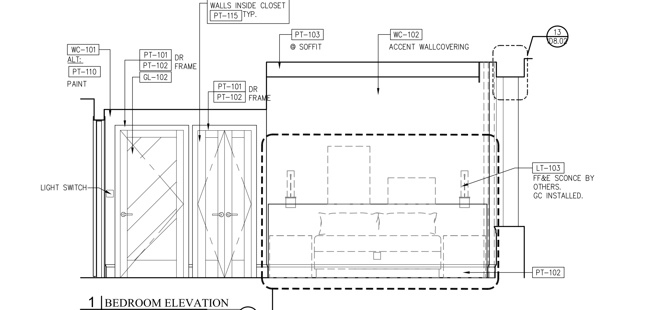
1 BEDROOM ELEVATION 3/8" = 1'-0"
