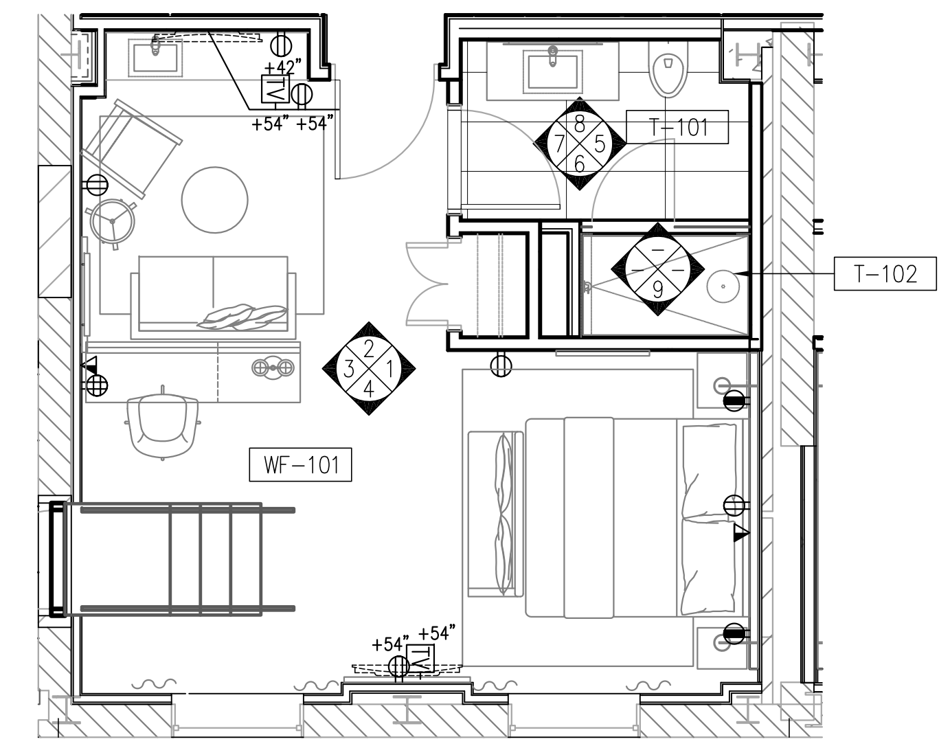
20 ROOM TYPE O FLOOR PLAN 1/4" = 1'-0"
